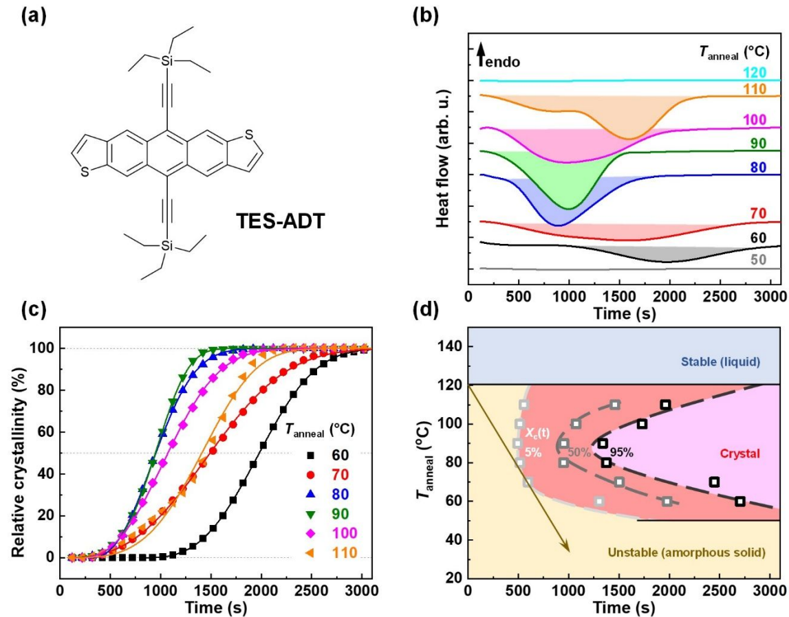
Figure 1. a) Chemical structure of TES-ADT. b) Isothermal DSC thermograms of TES-ADT recorded during annealing at various T_{\text{anneal}} . c) relative crystallinity X_c(t) as a function of time t (symbols) and best fits with the Avrami equation (solid lines). d) Time-temperature-transformation (TTT) diagram displaying the time for X_c(t) to reach 5%, 50% and 95%. The arrow represents the slowest constant-rate cooling process that results in a close to amorphous solid with X_c(t) \approx 5\% (cooling rate \approx -0.083 °C s -1 ).
