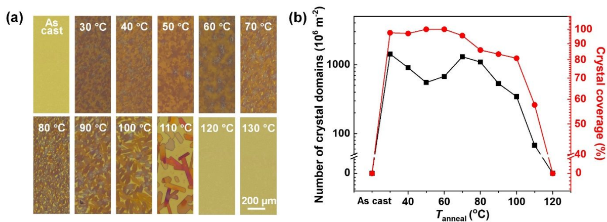
Figure 2. (a) Polarized optical microscopy images recorded with two polarizers placed at an angle of 45° (not fully crossed) of TES-ADT thin films annealed at various temperatures and (b) number of crystal domains per area and crystal coverage extracted from the optical micrographs.
