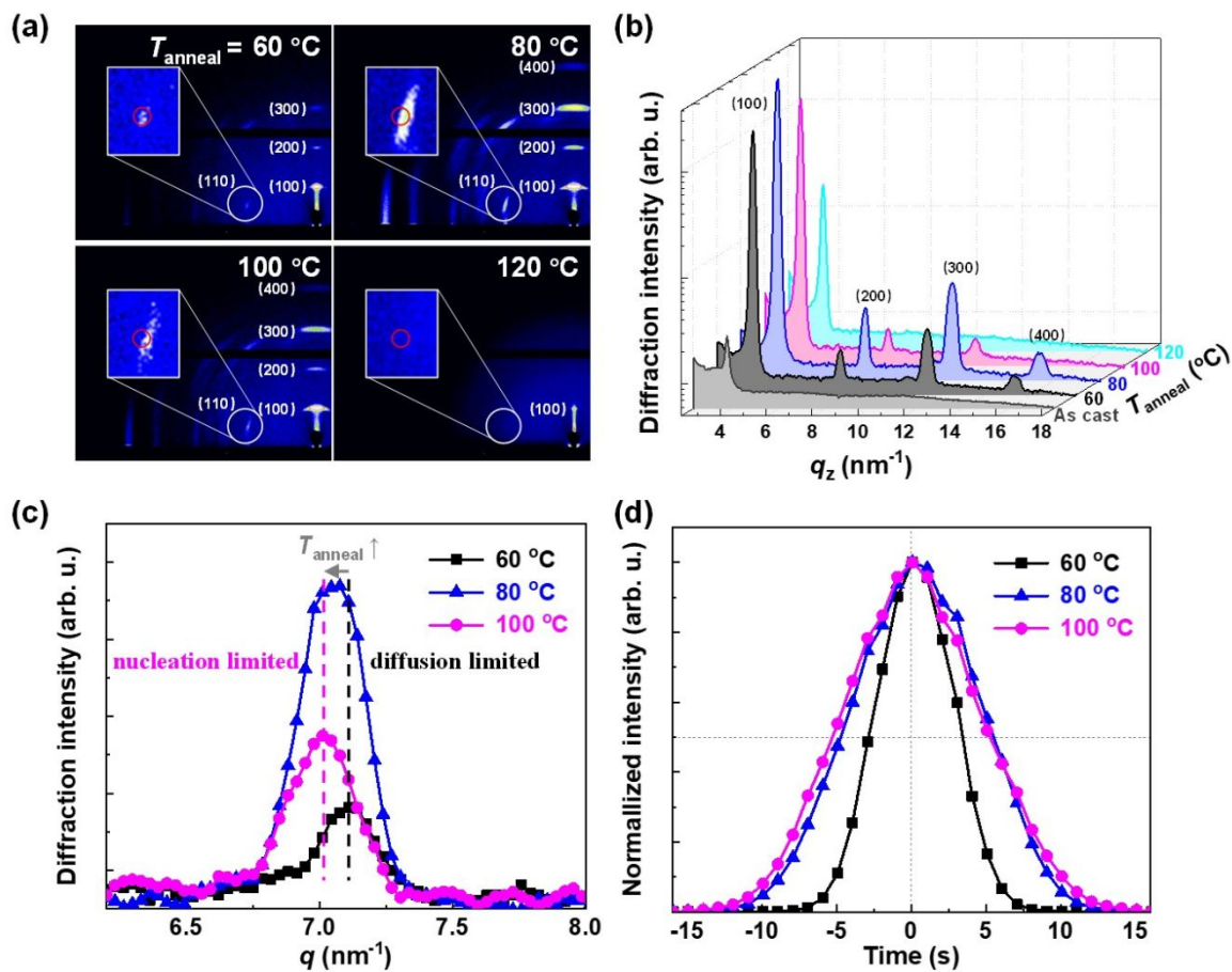
Figure 3. a) GIWAXS patterns of TES-ADT thin films annealed at various temperatures with the (110) diffractions highlighted and enlarged in the insets. b) Vertical line cuts of (a) depicting the out-of-plane ( l00 ) diffractions. c) Comparison of the (110) diffraction of thin films annealed in the diffusion limited (DL) and nucleation limited (NL) region, which gives rise to slight variations of the \gamma -phase. d) Azimuthal distribution of the (100) diffraction.
