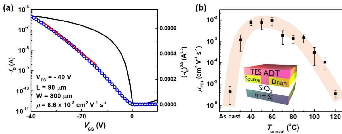
Figure 4. a) Transfer characteristics of a FET device with a TES-ADT active layer annealed at 60 °C. b) saturation mobility of FET devices ( \mu_{\text{FET}} ) annealed at various temperatures.
