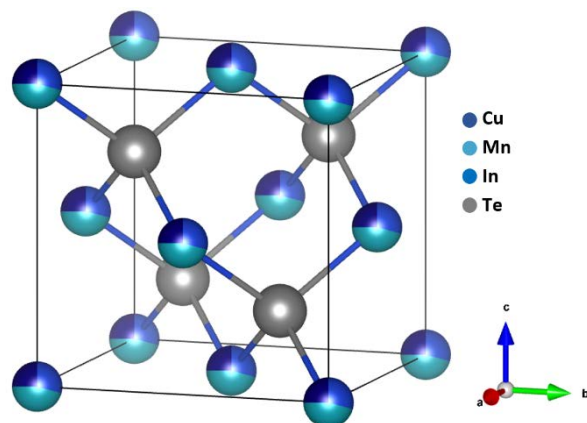
Figure 1. Crystal structure of \text{CuMnInTe}_4 .
