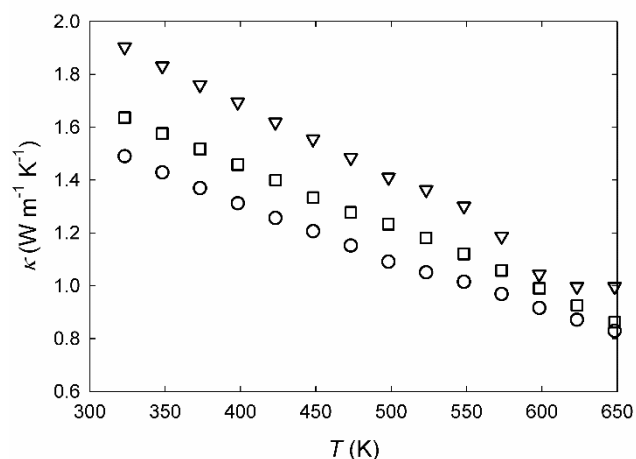
Figure 4. Temperature dependent \kappa for \text{CuMn}_2\text{InTe}_4 (circle), \text{Cu}_{1.2}\text{Mn}_{1.8}\text{InTe}_4 (triangle) and \text{Cu}_{1.3}\text{Mn}_{1.7}\text{InTe}_4 (square).
