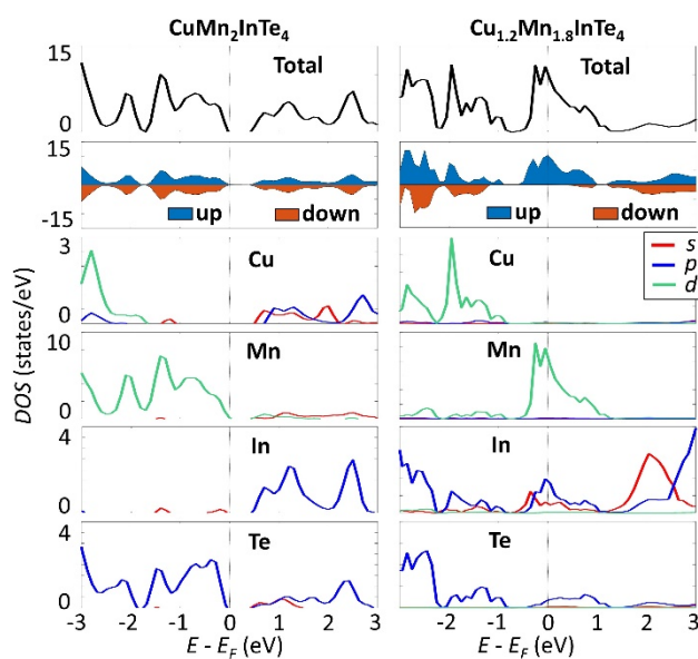
Figure 6. Total, spin-polarized, atomic and orbital projected density of states for \text{CuMn}_2\text{InTe}_4 and \text{Cu}_{1.2}\text{Mn}_{1.8}\text{InTe}_4 .
