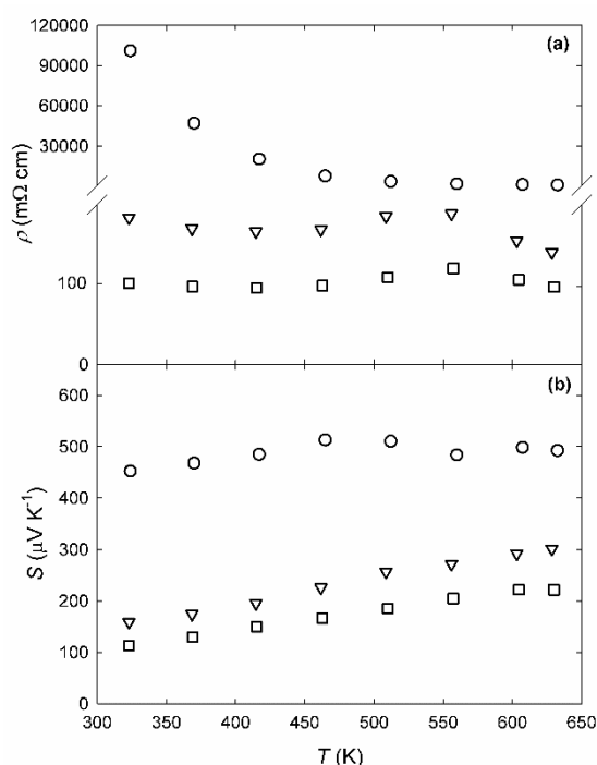
Figure 5. Temperature dependent (a) \rho and (b) S for \text{CuMn}_2\text{InTe}_4 (circle), \text{Cu}_{1.2}\text{Mn}_{1.8}\text{InTe}_4 (triangle) and \text{Cu}_{1.3}\text{Mn}_{1.7}\text{InTe}_4 (square).
