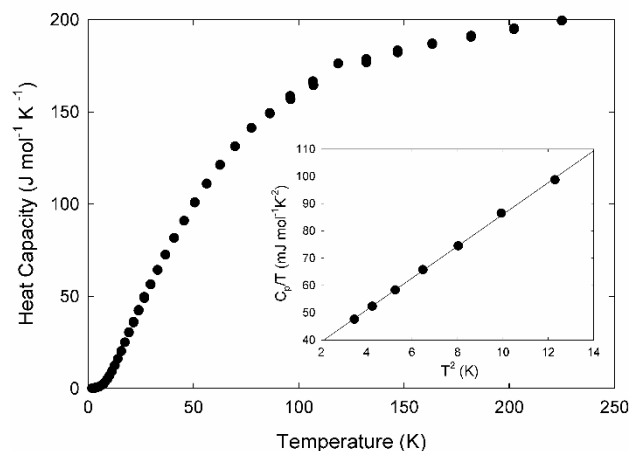
Figure 8. Temperature dependent C_p of \text{Cu}_{1.2}\text{Mn}_{1.8}\text{InTe}_4 . The inset shows C_p/T vs T^2 data at low temperatures with the solid line representing the C_p/T = \gamma + \beta T^2 relation.
