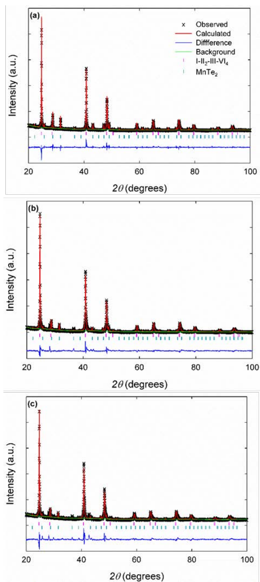
Figure 2. Powder XRD data for (a) CuMn 2 InTe 4 , (b) Cu 1.2 Mn 1.8 InTe 4 and (c) Cu 1.3 Mn 1.7 InTe 4 including profile fit, profile difference, profile residuals and Bragg positions.
