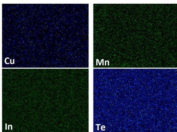
Figure 3. EDS elemental mapping images showing Cu, Mn, In and Te, illustrating the homogeneity of Cu 1.3 Mn 1.7 InTe 4 .
