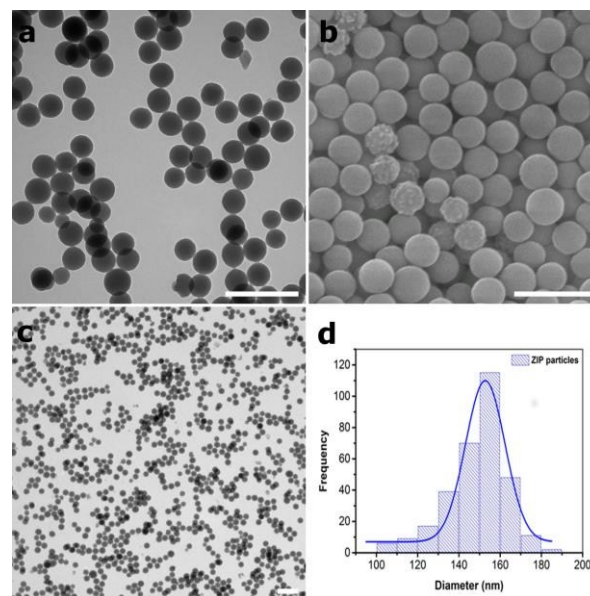
Fig. 2 (a), (b) and (c) TEM and SEM images of as-synthesized ZIP particles. Scale bars = 500 nm. (d) Particle size distribution of ZIP particles, d = 143 \pm 33 ; PDI = 0.07.
