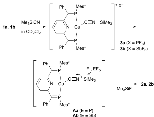
Scheme 2 Bond activation of \text{Me}_3\text{SiCN} promoted by 1a and 1b .
