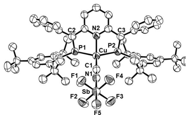
Fig. 2 ORTEP drawing of 2b with 50% probability ellipsoids. Hydrogen atoms are omitted for clarity. Selected bond distances (Å) and angles (deg): Cu-C1 = 1.886(7), Cu-P1 = 2.321(2), Cu-P2 = 2.310(2), Cu-N2 = 2.021(5), C1-N1 = 1.180(8), N1-Sb = 2.043(6), Sb-F1 = 1.843(4), Sb-F2 = 1.858(4), Sb-F3 = 1.849(4), Sb-F4 = 1.847(4), Sb-F5 = 1.861(5), P1-C2 = 1.690(6), P2-C3 = 1.705(6), N-Cu-C1 = 126.2(2), P1-Cu-P2 = 135.95(7), Cu-C1-N1 = 178.5(6), C1-N1-Sb = 174.5(6), N1-Sb-F1 = 88.3(2), N1-Sb-F2 = 90.2(2), N1-Sb-F3 = 89.1(2), N1-Sb-F4 = 87.4(2), N1-Sb-F5 = 178.6(2).
