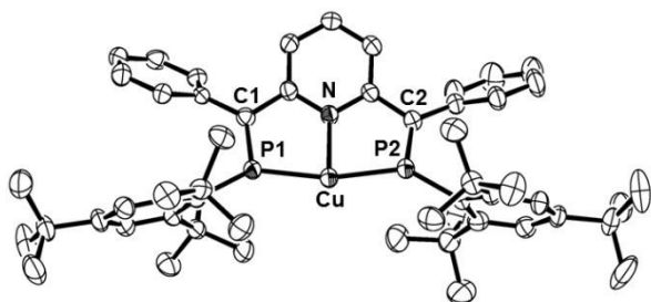
Fig. 1 ORTEP drawing of 1c with 50% probability ellipsoids. Hydrogen atoms, \text{BAR}^{\text{F}_4} anion and a crystal solvent ( \text{CH}_2\text{Cl}_2 ) are omitted for clarity. Selected bond distances (Å) and angles (deg): Cu–P1 = 2.206(1), Cu–P2 = 2.216(1), Cu–N = 2.074(3), P1–C1 = 1.691(4), P2–C2 = 1.711(4), P1–Cu–N = 84.5(1), P2–Cu–N = 84.5(1), P1–Cu–P2 = 167.09(5).
