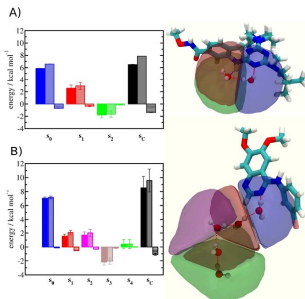
Fig 10. Spatial decomposition of the changes in hydration energetics within the GCT monitored regions. The monitored region depicted in figure 7 and 8 was broken down into sub-regions for the rc = full protocol simulations. For each sub-region, the relative hydration free energy \Delta\Delta G_{hyd}(AP \rightarrow BP, S_{BP}, S_{AP}, r_c) , relative hydration enthalpy \Delta\Delta H_{hyd}(AP \rightarrow BP, S_{BP}, S_{AP}, r_c) and relative hydration entropy -T\Delta\Delta S_{hyd}(AP \rightarrow BP, S_{BP}, S_{AP}, r_c) are depicted as bars (left). The contributions from the full region s_c are shown in black. The right panel depicts the localisation of each sub-region. A) p38 MAP kinase. B) EGFR kinase.
