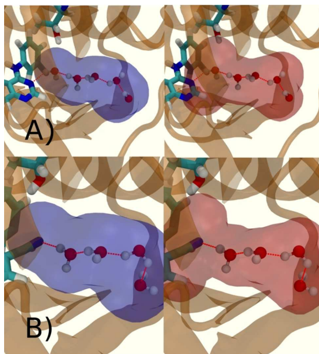
Fig 8. Representation of GCT monitored regions in EGFR kinase (A) In complex with 5 (B) in complex with 6 . Regions s_{AP} and s_{BP} are depicted by the transparent blue volumes at r_c = full conditions (left) while s_{AP} and s_{BP} are depicted by red transparent volumes in r_c = bb (right) conditions. X_{medoid} = 4 \text{ \AA} in both cases. Relevant hydrogen-bonding interactions between protein residues, water molecules and ligands are depicted by red-dotted lines.
