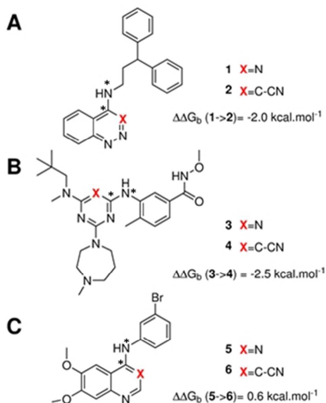
Fig 1. Structures of the three pairs of ligands considered in this study. A) scytalone dehydratase, B) p38 \alpha MAP kinase C) EGFR kinase. Estimates of the experimental relative binding affinities are also shown. The star symbol denotes atoms used to define positional restraints (see methods).
