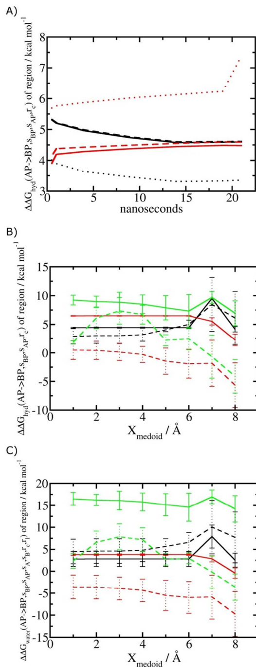
Fig 5. Convergence of hydration energetics and water reorganisation energetics for protein-ligand complexes. (A) Convergence of hydration energetics (equation 1) with respect to trajectory duration for scytalone dehydratase. Results in black are for r_c = full , and in red for r_c = bb . The solid line is for X_{medoid} = 1 Å, the dashed line for X_{medoid} = 4 Å, and the dotted line for X_{medoid} = 8 Å. (B) Hydration energetics as a function of X_{medoid} using the full trajectories for scytalone dehydratase (black) p38 MAP kinase (red), and EGFR kinase (green). Solid lines are the results obtained with the r_c = full protocol and dotted lines are the results obtained with the r_c = bb protocol. (C) Same as B) but for the water reorganisation energy (eq 2) using r_l = full, X_{vdw} = 6 Å or r_l = rot, X_{cubic} = 10 Å.
