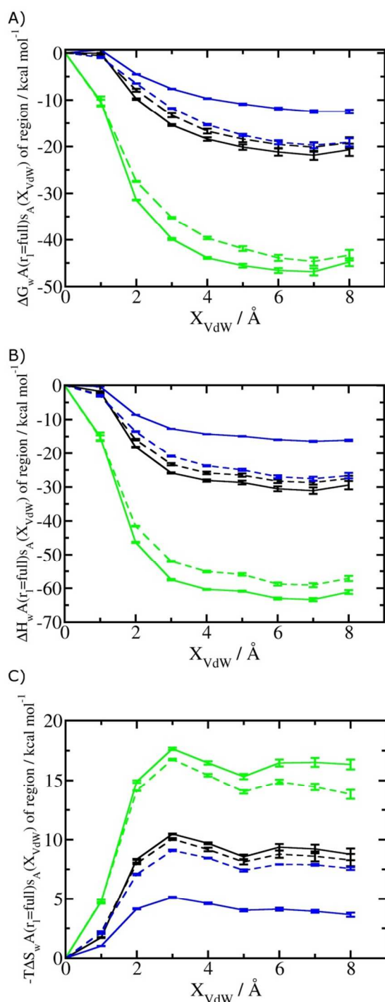
Fig. 3 Ligand hydration energetics with the full restraints protocol (A) Hydration free energies \Delta G_{w,A}^{SA}(r=\text{full})_A(X_{\text{vdW}}) , (B) Hydration enthalpies \Delta H_{w,A}^{SA}(r=\text{full})_A(X_{\text{vdW}}) , and (C) Hydration entropies -T\Delta S_{w,A}^{SA}(r=\text{full})_A(X_{\text{vdW}}) . Black lines are for the scytalone dehydratase ligands 1 (solid) and 2 (dashed). Green lines are for the p38 MAP kinase ligands 3 (solid) and 4 (dashed). Blue lines are for the EGFR kinase ligands 5 (solid) and 6 (dashed). Error bars represent the standard error of the mean computed from triplicate independent simulations.
