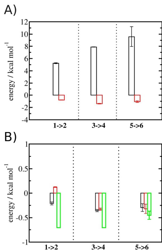
Fig 9. Thermodynamic signature of the changes in the hydration energetics of the three protein-ligand complexes. (A) Enthalpy changes \Delta\Delta H_{hyd}(AP \rightarrow BP, S_{BP}, S_{AP}, r_c) are shown as empty ( r_c = full ) or shaded ( r_c = bb ) black histograms. Entropy changes -T\Delta\Delta S_{hyd}(AP \rightarrow BP, S_{BP}, S_{AP}, r_c) are shown as empty ( r_c = full ) or shaded ( r_c = bb ) red histograms. (B) Decomposition of the entropy changes in vibrational entropy -T\Delta\Delta S_{vib}(AP \rightarrow BP, S_{BP}, S_{AP}, r_c) (black), librational entropy -T\Delta\Delta S_{lib}(AP \rightarrow BP, S_{BP}, S_{AP}, r_c) (red) and orientational entropy -T\Delta\Delta S_{ori}(AP \rightarrow BP, S_{BP}, S_{AP}, r_c) (green) components. Error bars represent the standard error of the mean from three replicates.
