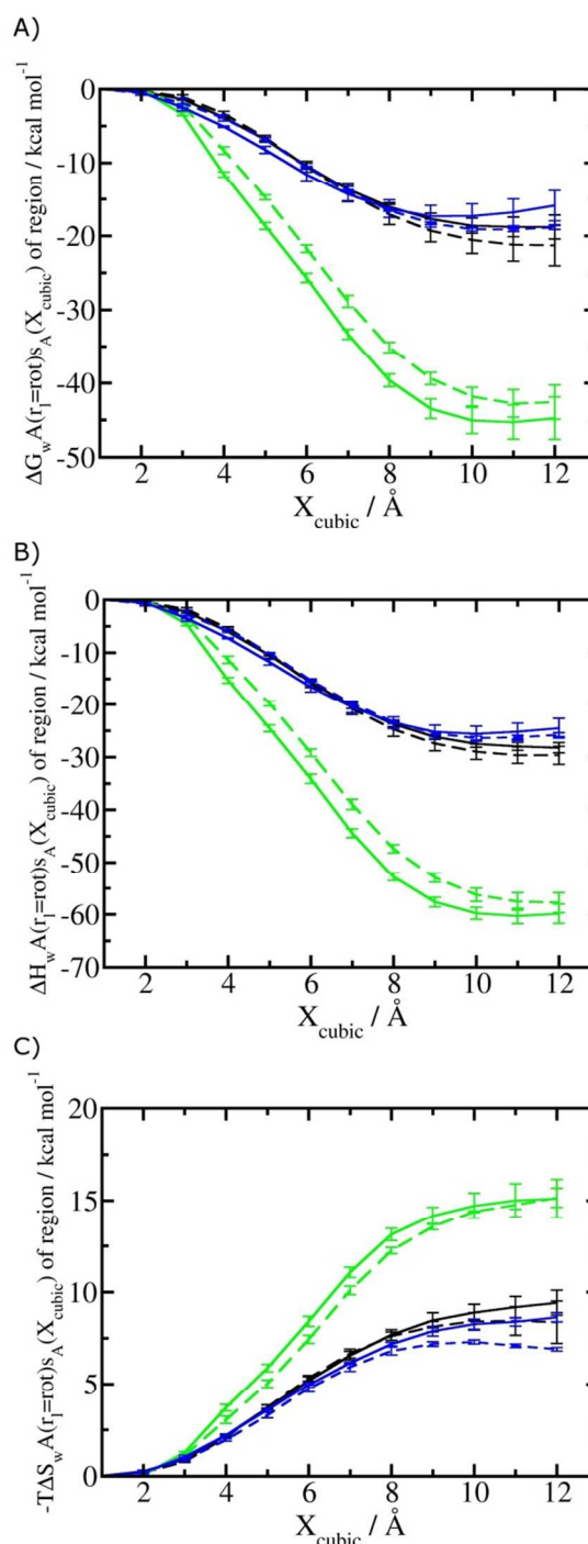
Fig. 4 Ligand hydration energetics with the rigid body rotation restraints protocol (A) Hydration free energies \Delta G_{w,A}^{SA}(r=\text{rot})_A(X_{\text{cubic}}) , (B) Hydration enthalpies \Delta H_{w,A}^{SA}(r=\text{rot})_A(X_{\text{cubic}}) , and (C) Hydration entropies -T\Delta S_{w,A}^{SA}(r=\text{rot})_A(X_{\text{cubic}}) . Black lines are for the scytalone dehydratase ligands 1 (solid) and 2 (dashed). Green lines are for the p38 MAP kinase ligands 3 (solid) and 4 (dashed). Blue lines are for the EGFR kinase ligands 5 (solid) and 6 (dashed). Error bars represent the standard error of the mean computed from triplicate independent simulations.
