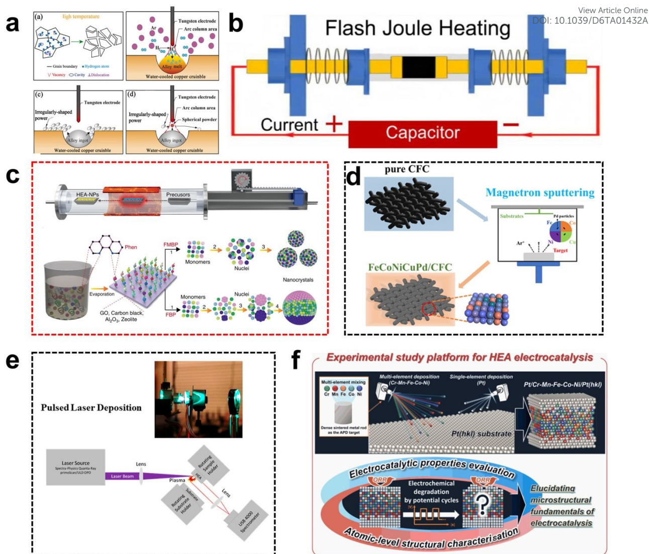
Figure 10 (a) Schematic diagram of the hydrogen plasma–arc melting method. Reproduced with permission [101]. Copyright 2024, Elsevier. (b) Flash Joule heating device diagram. Reproduced with permission [104]. Copyright 2025, Elsevier. (c) Schematic diagram of the FMBP experimental setup for the synthesis of HEA-NPs. Reproduced with permission [106]. Copyright 2020, Springer Nature. (d) Schematic illustration of key FeCoNiCuPd thin film fabrication steps. Reproduced with permission [112]. Copyright 2022, Elsevier. (e) Schematic illustration of pulsed laser deposition. Reproduced with permission [116]. Copyright 2024, American Chemical Society. (f) Schematic illustration of the experimental study platform of the HEA electrocatalysis model surface via multiple arc-plasma depositions. Reproduced with permission [118]. Copyright 2023, Springer Nature.
