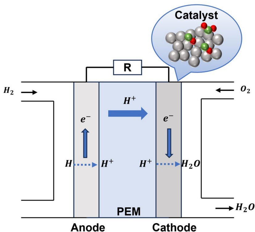
Figure 2 Schematic diagram of the fuel cell and ORR in acidic media
