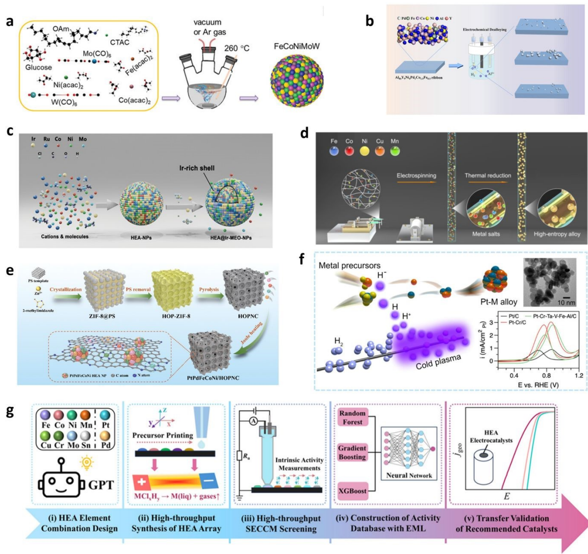
Figure 11 (a) Schematic diagram of the colloidal synthesis process used to produce FeCoNiMoW nanoparticles. Reproduced with permission [81]. Copyright 2023, Wiley-VCH GmbH. (b) Schematic of the preparation of the Ni-Pd-Co-Fe catalyst. Reproduced with permission [129]. Copyright 2025, Royal Society of Chemistry. (c) Schematic of the prepared HEA and HEA@Ir-MEO. Reproduced with permission [131]. Copyright 2024, Wiley-VCH GmbH. (d) Synthesis procedure of HEA/CNF hybrid nanomaterials through a polymer fiber nanoreactor. Reproduced with permission [133]. Copyright 2023, Royal Society of Chemistry. (e) Schematic illustration of the preparation of PtPdFeCoNi/HOPNC. Reproduced with permission [135]. Copyright 2025, Wiley-VCH GmbH. (f) Schematic illustration of the
