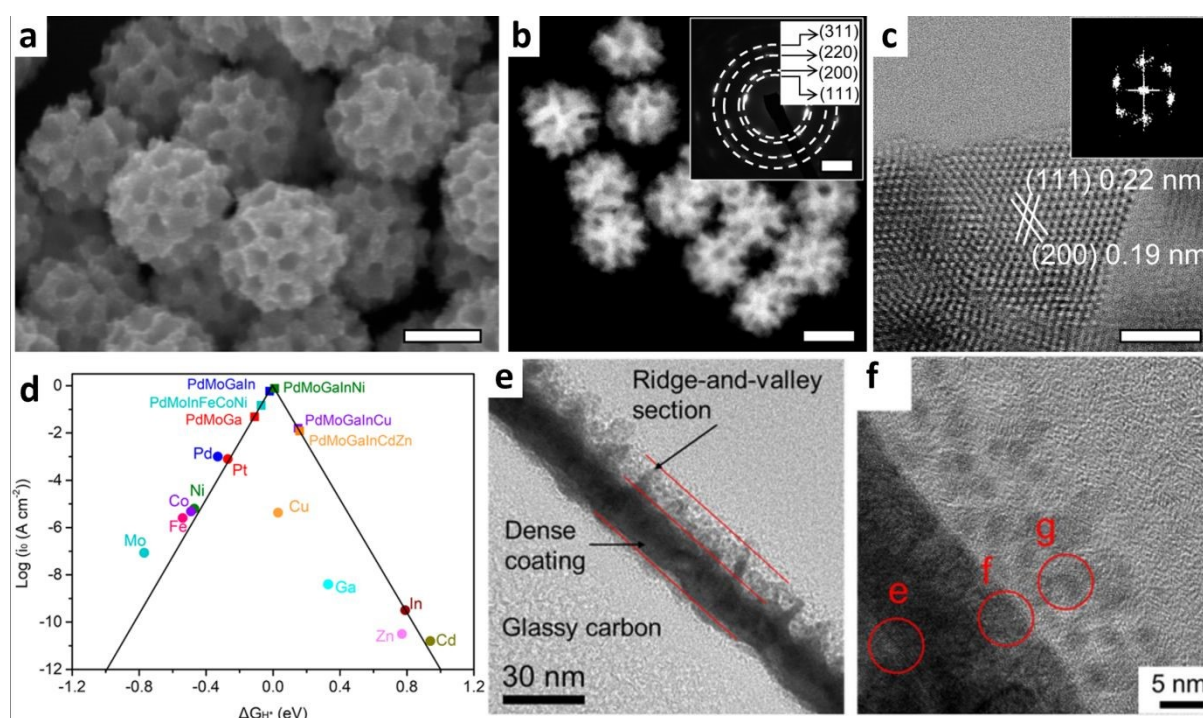
Figure 9 (a) SEM image (scale bar: 100 nm) and (b) HAADF-STEM image (scale bar: 100 nm). Insets: corresponding SAED patterns (scale bar: 5 \text{ nm}^{-1} ). (c) HRTEM (scale bar: 2 nm) (FFT patterns are shown in the inset) of the PtPdRhRuCu mesoporous nanospheres. Reproduced with permission [62]. Copyright 2023, Springer Nature. (d) A plot constructed from experimentally derived exchange current densities and computationally calculated hydrogen binding energies of various single elements and HEAs. Reproduced with permission [65]. Copyright 2022, American Chemical Society. (e) (f) HR-TEM images of the cross-sectional and subsurface areas of \text{Ir}_{20.3}\text{Pd}_{16.3}\text{Pt}_{8.6}\text{Rh}_{26.1}\text{Ru}_{28.7}/\text{GC} . Reproduced with permission [66]. Copyright 2024, Royal Society of Chemistry.
