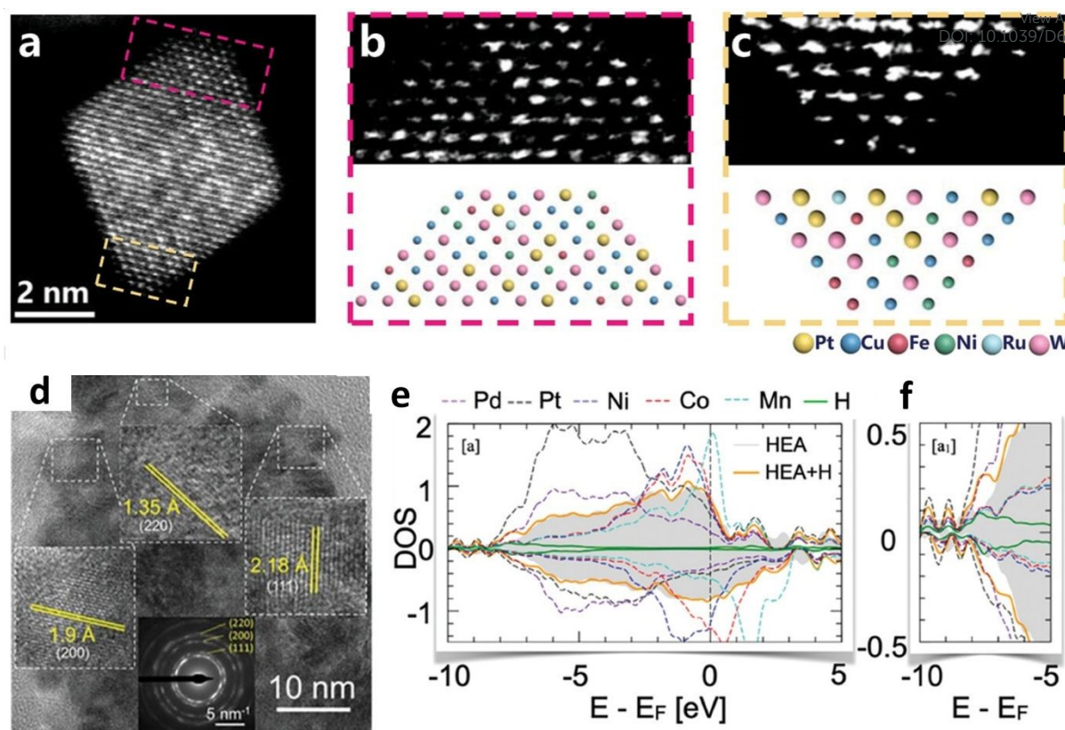
Figure 7 (a)-(c) HAADF-STEM image and atomically resolved HAADF-STEM images of Ru-doped (0.2 at %) \text{Pt}_{24.8}\text{Fe}_{12.7}\text{Ni}_{7.1}\text{Cu}_{34.5}\text{W}_{20.8} HEA nanocrystals. Corresponding simulated atomic images contained in (b) and (c). Reproduced with permission [50]. Copyright 2024, Wiley-VCH GmbH. (d) HRTEM image showing the d-spacing value of PtPdNiCoMn. (e), (f) DFT calculation of the PDOS of PtPdNiCoMn and the magnified region. Reproduced with permission [53]. Copyright 2025, Wiley-VCH GmbH.
