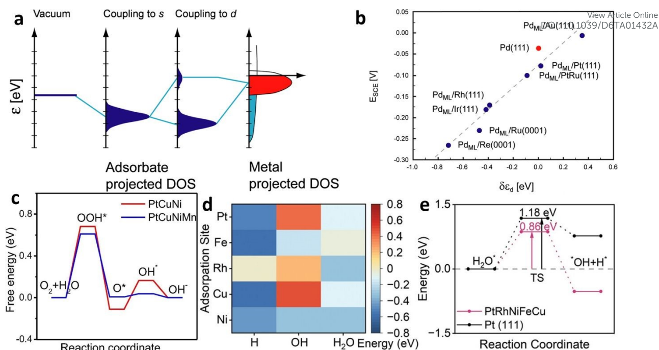
Figure 5 (a) Schematic illustration of bond formation between the valence level and the s and d states of a TM surface. Adapted with permission [29]. Copyright 2011, National Academy of Science, USA. Reproduced with permission [30]. Copyright 2005, Wiley-VCH GmbH. (b) Electrochemically measured changes in the hydrogen adsorption energy ( E_{SCE} ) are shown to scale well with the calculated shift in the d-band center ( \delta\epsilon_d ). Reproduced with permission [30]. Copyright 2005, Wiley-VCH GmbH. (c) Free energy profiles for various ORR steps with the CuNiMnPt and CuNiPt catalysts. Reproduced with permission [43]. Copyright 2020, Elsevier. (d) Adsorption preferences for water and intermediates on different metal sites of the HEA. (e) Activation energies of water dissociation of PtRhNiFeCu and Pt. Reproduced with permission [45]. Copyright 2024, Wiley-VCH GmbH.
