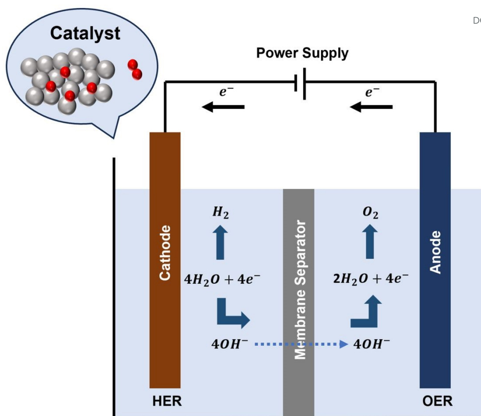
Figure 1 Schematic diagram of water electrolysis and HER in alkaline media
