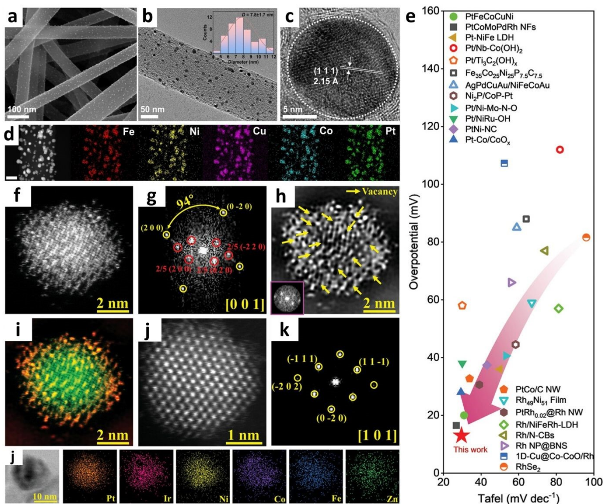
Figure 6 (a), (b), (c), and (d) SEM, TEM, HRTEM, HAADF-STEM images and EDS mapping of FeNiCuCoPt on carbon nanofibers. (Scale bar: 50 nm). Reproduced with permission [48]. Copyright 2024, Wiley-VCH GmbH. (e) Overpotentials at 10 \text{ mA cm}^{-2} and Tafel slopes for various HEAs for the alkaline HER. Reproduced with permission [45]. Copyright 2024, Wiley-VCH GmbH. (f) HR-STEM image of a PtIrNiCoFeZn HEA nanoparticle. (g) FFT pattern of (f). (h) IFFT image of the corresponding FFT pattern (inset). (i) Color-mixed images of (f) and (h); (f) is set as green, and (h) is set as red. (j) HR-STEM image of a PtIrNiCoFe HEA nanoparticle. (k) FFT pattern of (j). (l) STEM-EDS mapping of a PtIrNiCoFeZn HEA. Reproduced with permission [49]. Copyright 2024, Wiley-VCH GmbH.
