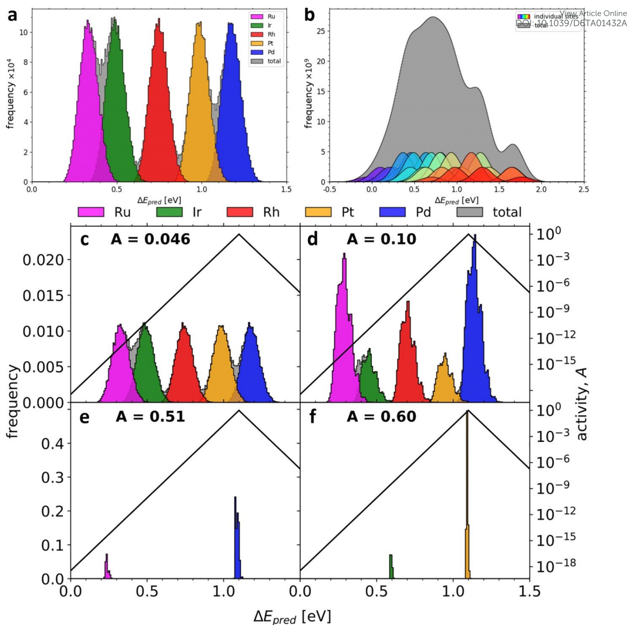
Figure 8 (a)(b) Predicted adsorption energies for OH* and O*. (c), (d), (e), and (f) Distributions of the adsorption energies for IrPdPtRhRu, Ir 10.2 Pd 32 Pt 9.3 Rh 19.6 Ru 28.9 , Pd 81.7 Ru 18.3 and Ir 17.5 Pt 82.5 , respectively. Reproduced with permission [56]. Copyright 2019, Cell Press.
