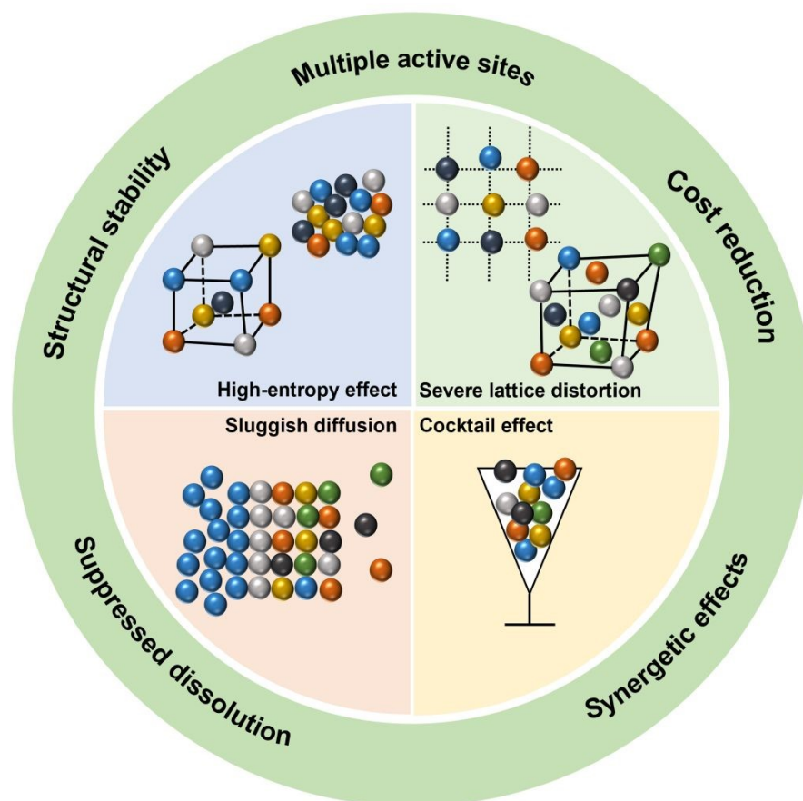
Figure 3 Four core effects of HEAs
