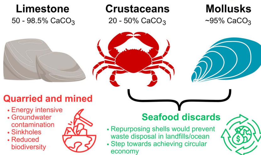
Fig. 2 Natural sources of \text{CaCO}_3 include limestone and calcifiers (e.g., crustaceans & mollusks). Prepared with Canva.
