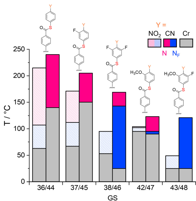
Fig. 5 Transitional behaviour of GS36–48, comparing cyano and nitro terminal groups. Cr indicates the temperature at which the sample recrystallises on supercooling using the polarised optical microscope.
