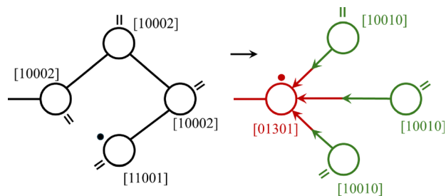
Fig. 4 New cycle representation, formation of a cycle of size 4. The radical on the chain head attacks a vinyl group on the 4th unit. This creates in- and outgoing edges as expressed by the changes of the species vectors, [v, r, i, o, u] . The two reacting units change, but also the non-reacting intermediate units.
