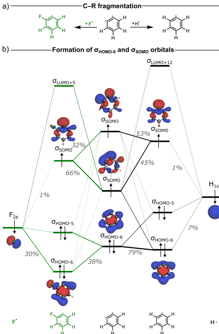
Fig. 5 (a) Fragmentation of the C–R bond (R = F versus H). (b) Qualitative MO diagram showing the formation of the \sigma_{\text{SOMO}} and \sigma_{\text{HOMO-6}} of the aryl radical ( C_6RH_4 ) from the interaction of C_6H_4^{\cdot\cdot} + R\cdot . SFO gross Mulliken contributions (in gray) are shown only for \sigma_{\text{SOMO}} and \sigma_{\text{HOMO-6}} ; for details on the other orbitals, see Fig. S8 and Table S4. Computed at ZORA-BLYP-D3(BJ)/TZ2P.
