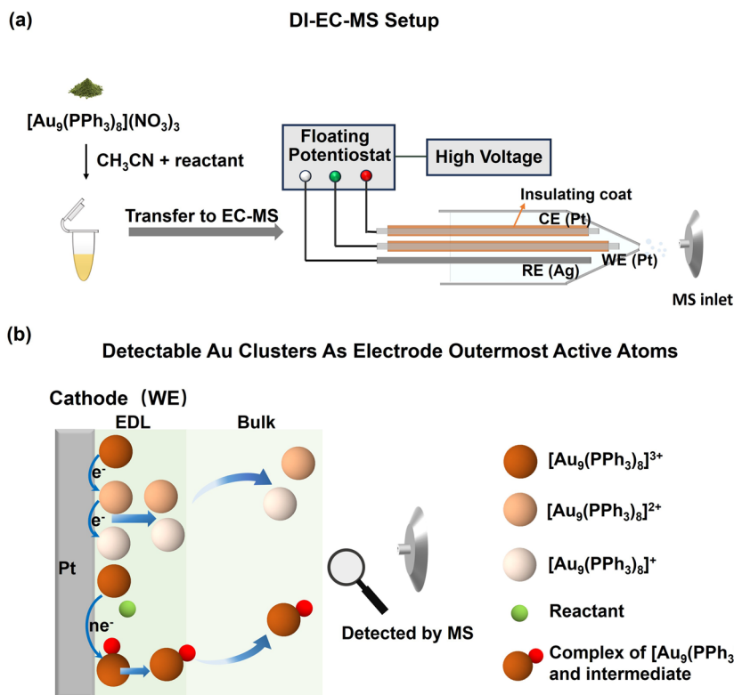
Fig. 1 (a) Schematic illustration of the DI-EC-MS. In the experiment, [\text{Au}_9(\text{PPh}_3)_8](\text{NO}_3)_3 and the target EC reaction substrates are dissolved in acetonitrile and then transferred into the online EC cell for continuous reaction monitoring. (b) Schematic illustration of detachable [\text{Au}_9(\text{PPh}_3)_8]^{3+} clusters acting as the outermost active atomic layer of the working electrode. The negatively polarized Pt electrode electrostatically attracts the positively charged [\text{Au}_9(\text{PPh}_3)_8]^{3+} clusters, leading to their enrichment on the electrode surface. After reduction of the clusters and the substrate molecules, the decreased positive charge weakens the interaction between the gold clusters and the interface, causing the clusters to desorb from the electrode surface and enter the solution.
