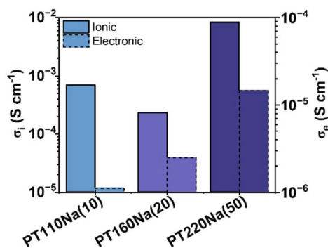
Fig. 5 Ionic and electronic conductivity at 60 °C for Na-CBEs with varying P3HT wt%: 10 (PT110Na above), 20 wt% P3HT, DP_{P3HT} = 160 and 50 wt% P3HT, DP_{P3HT} = 220 .
