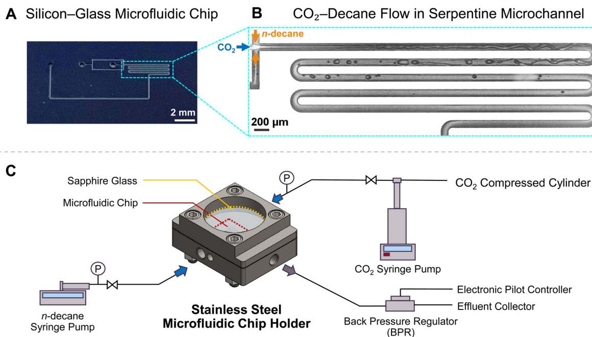
Fig. 1 (A) Photograph of the fabricated silicon–glass microfluidic chip. (B) Microscopy image showing the \text{CO}_2 –decane flow in a serpentine microchannel. Scale bar: 200 \mu\text{m} . (C) Schematics of the microfluidic experimental setup. \text{CO}_2 and n -decane were injected using two separate high-pressure syringe pumps. Center: 3D model of the stainless steel microfluidic chip holder with a sapphire viewing window and the microfluidic chip positioned beneath it. Backpressure was controlled using a backpressure regulator with an electronic pilot controller.
