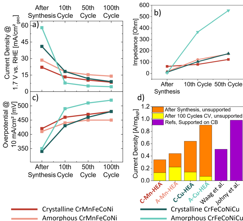
Fig. 6 OER activity of amorphous/crystalline CrMnFeCoNi and CrFeCoNiCu HEA NPs, showing extracted current densities at 1.7 V vs. RHE (a) and overpotentials at 10 \text{mA}/\text{cm}^2_{\text{geo}} (c) from linear sweep voltammetry experiments. (b) Impedance of HEA NPs with different states of the nanoparticle surface (after synthesis, after 10 CV cycles, and after 50 cycles) and (d) comparison of OER current densities extracted at 1.7 V vs. RHE: crystalline and amorphous Mn-containing HEA NPs (C-Mn-HEA and A-Mn-HEA) compared to crystalline and amorphous Cu-containing HEA NPs (C-Cu-HEA and A-Cu-HEA) as well as reference values of CB-supported HEA NPs, reported by Waag et al. 39 (crystalline CrMnFeCoNi HEA NPs obtained via ps-LAL in ethanol) and Johny et al. 41 (amorphous CrMnFeCoNi HEA NPs obtained via ns-LAL in acetonitrile).
