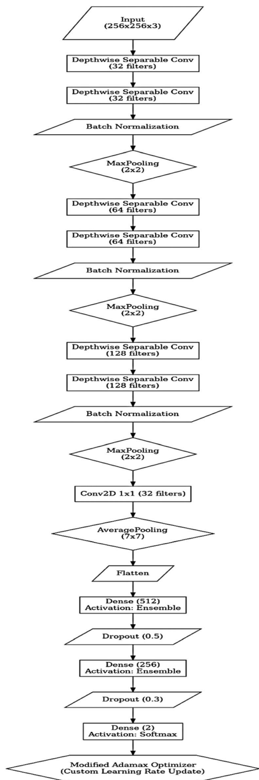
Fig. 1 Flow chart of the developed L-Net model.
