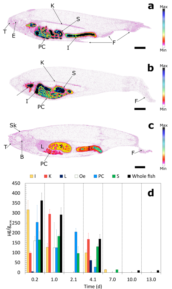
Fig. 3 Quantitative whole-body autoradiography analysis of [ ^{14}\text{C} ]nPS _{20} in O. mykiss following single-day high-dose exposure to 250 ng \text{g}_{\text{w.w.}}^{-1} at (a) 0.2 day, (b) 1 day, and (c) 4 days post-ingestion. Colour scales represent linear signal-to-noise (S/N) ratios; scale bars = 1 cm. Corresponding histological sections are provided in Fig. S7. (d) Organ-specific [ ^{14}\text{C} ]nPS _{20} quantification ( \mu\text{g}_{\text{C}} \text{g}_{\text{w.w.}}^{-1} ) above the LOD ( 9.53 \times 10^{-4} \mu\text{g}_{\text{C}} \text{g}_{\text{w.w.}}^{-1} ) and LOQ ( 2.89 \times 10^{-3} \mu\text{g}_{\text{C}} \text{g}_{\text{w.w.}}^{-1} ). Panels (a-d) show [ ^{14}\text{C} ]nPS _{20} only; [ ^{14}\text{C} ]nPS _{250} signals were GI-confined and below LOQ in systemic tissues at these time points (see Fig. S6, Table S2). Error bars represent inter-section variability ( n = 12 ). Abbreviations: B (bone), E (eye), F (fin), Gi (gills), I (intestine), K (kidney), L (liver), M (muscle), Oe (oesophagus), PC (pyloric caeca), Sk (skin), S (stomach), T (teeth).
