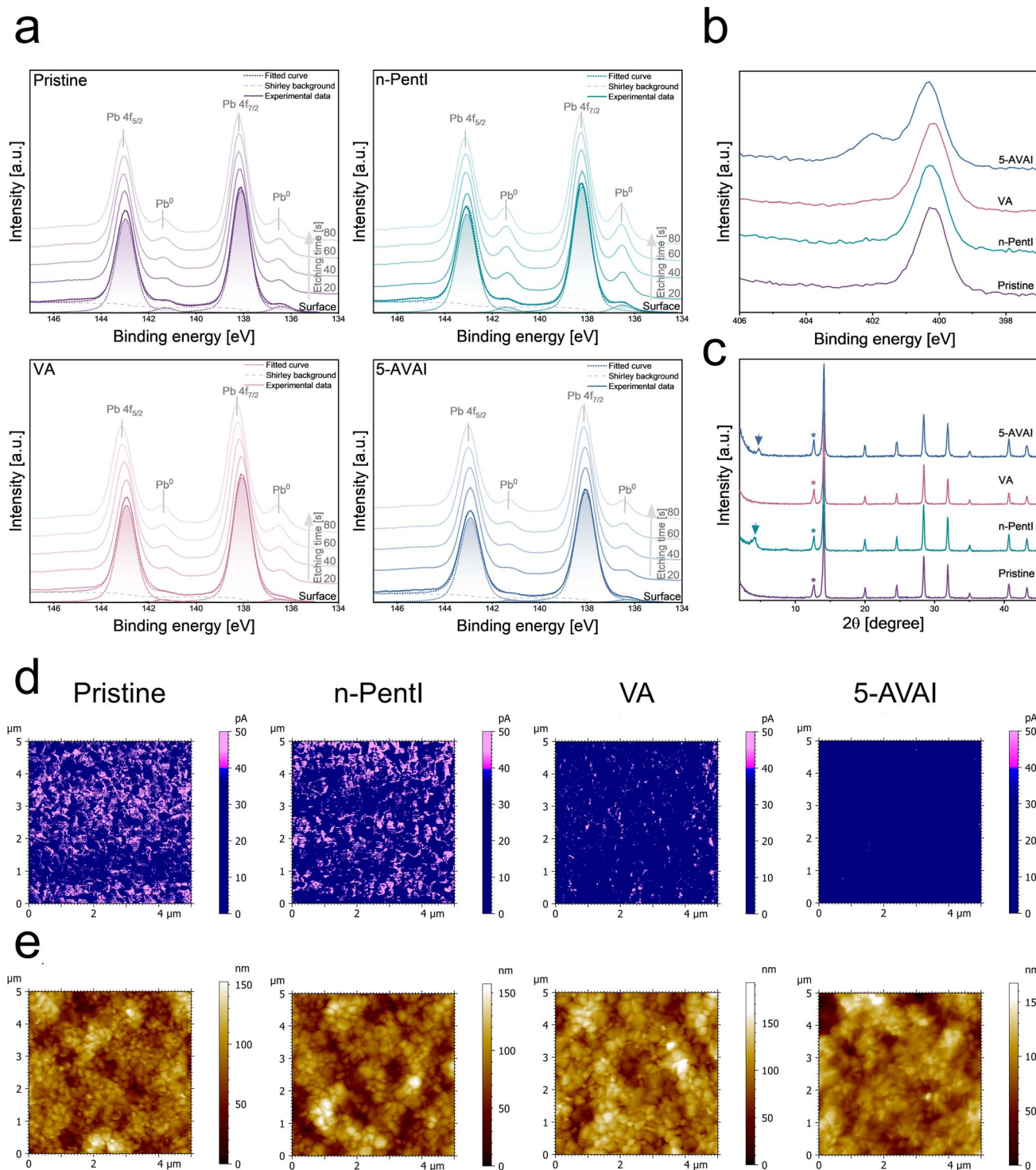
Fig. 2 Structural, compositional, and morphological characterization. XPS elemental scans of (a) Pb 4f and (b) N 1s. (c) XRD patterns of pristine and surface-modified perovskite thin films ( \text{Pb}_2 peaks at 2\theta = 12.5^\circ are marked by asterisks). (d) C-AFM images of the perovskite films. (e) Representative AFM images showcasing the topography of the perovskite films at 5 \mu\text{m} \times 5 \mu\text{m} .
