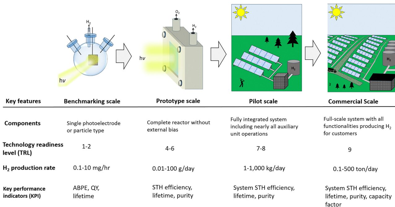
Fig. 4 Progression of PEC technology from materials development at benchmarking scale to commercial applications.
