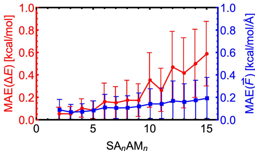
Fig. 6 Absolute error distributions of the modelled energies and force components for the SA_nAM_n clusters trained at the B97-3c level. The error bars show the standard deviation. Adapted from Kubečka et al. , 2024. 22 Adapted from ref. 22 with permission from the Royal Society of Chemistry, copyright 2024. Permission conveyed through Copyright Clearance Center.
