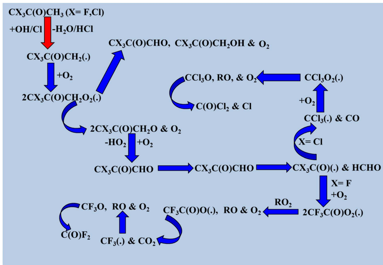
Scheme 13 Degradation process of \text{CHX}_2\text{C(O)CH}_3 ( \text{X} = \text{F} and \text{Cl} ).
