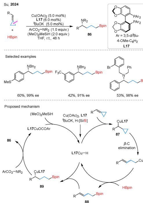
Scheme 21 Copper-catalyzed asymmetric borylmination of BCPs.
