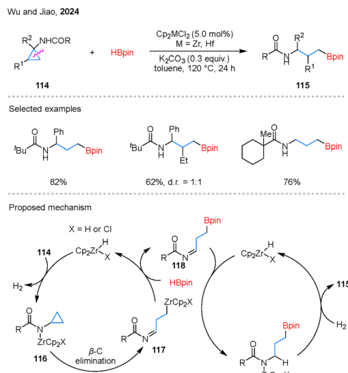
Scheme 26 Catalyzed hydroborylation of CPAs by earth-abundant group IV metals.
