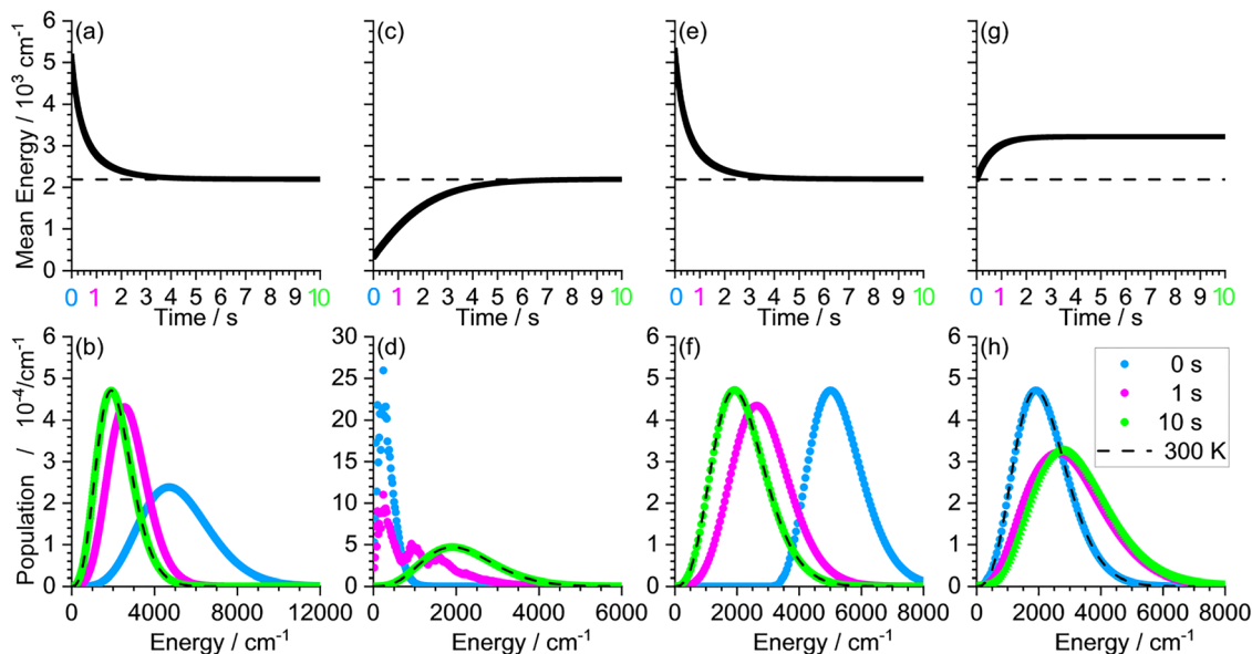
Fig. 8 MEM of \text{C}_6\text{H}_{23}\text{COO}^- simulating changes in internal energy in a 300 K environment: (a) and (b) cooling of an initial 500 K population; (c) and (d) heating of an initial 100 K population; (e) and (f) equilibration of a 300 K population after absorption of a 3091.43\text{ cm}^{-1} photon; (g) and (h) IRMPD experiment with absorption of 1694.44\text{ cm}^{-1} photons at a rate of 1 photon per second.
