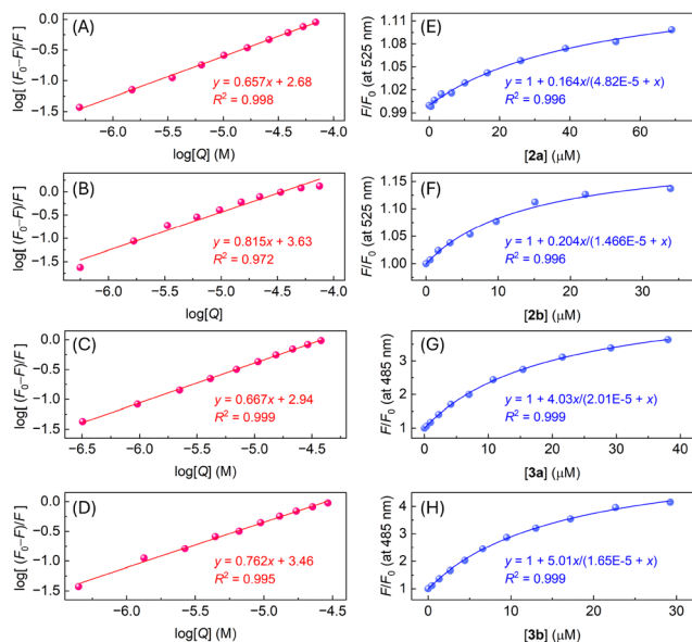
Fig. 13 Fluorescence titration data for compounds 2a (A), 2b (B), 3a (C), and 3b (D) fitted to the double-logarithmic model (eqn (2)). Fluorescence titration data for compounds 2a (E), 2b (F), 3a (G), and 3b (H) fitted to a 1 : 1 binding isotherm (eqn (3)).
