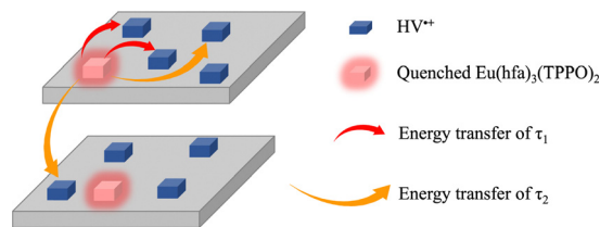
Fig. 10 Schematic diagram of energy transfer between \text{HV}^{\bullet+} and \text{Eu}(\text{hfa})_3(\text{TPPO})_2 between STN layers.
