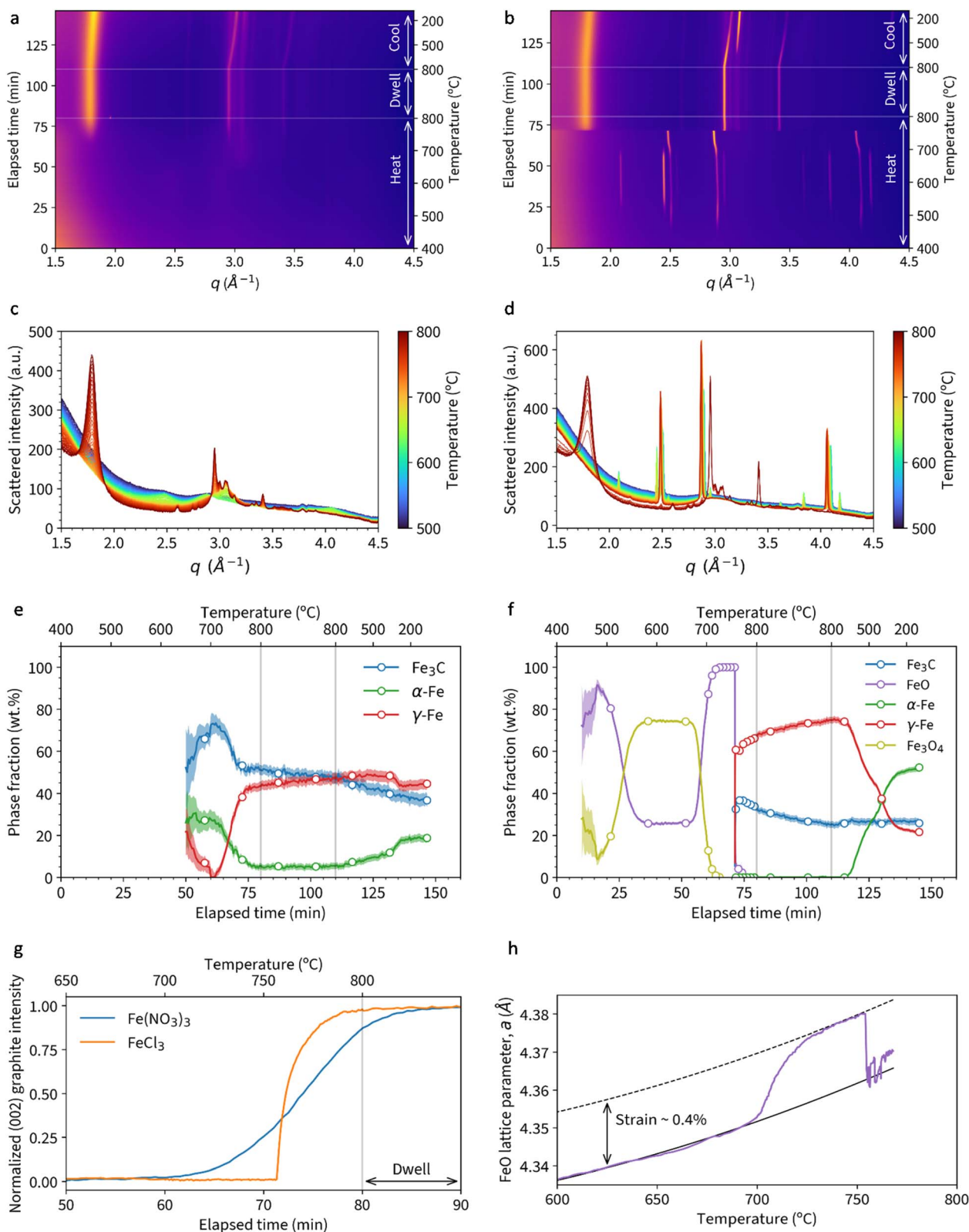
Fig. 2 Heatmaps of WAXS data for samples of (a) cellulose + \text{Fe}(\text{NO}_3)_3 and (b) cellulose + \text{FeCl}_3 heated to 800\text{ }^{\circ}\text{C} under nitrogen. Also diffraction data for (c) cellulose + \text{Fe}(\text{NO}_3)_3 and (d) cellulose + \text{FeCl}_3 with an additional panel showing the temperature for each pattern during heating to 800\text{ }^{\circ}\text{C} . Phase fractions extracted from Rietveld refinement of data for (e) cellulose + \text{Fe}(\text{NO}_3)_3 and (f) cellulose + \text{FeCl}_3 . A plot of (g) normalised graphite (002) peak intensity vs. time and temperature. (h) Plot showing expansion of FeO lattice parameter a with increasing temperature.
