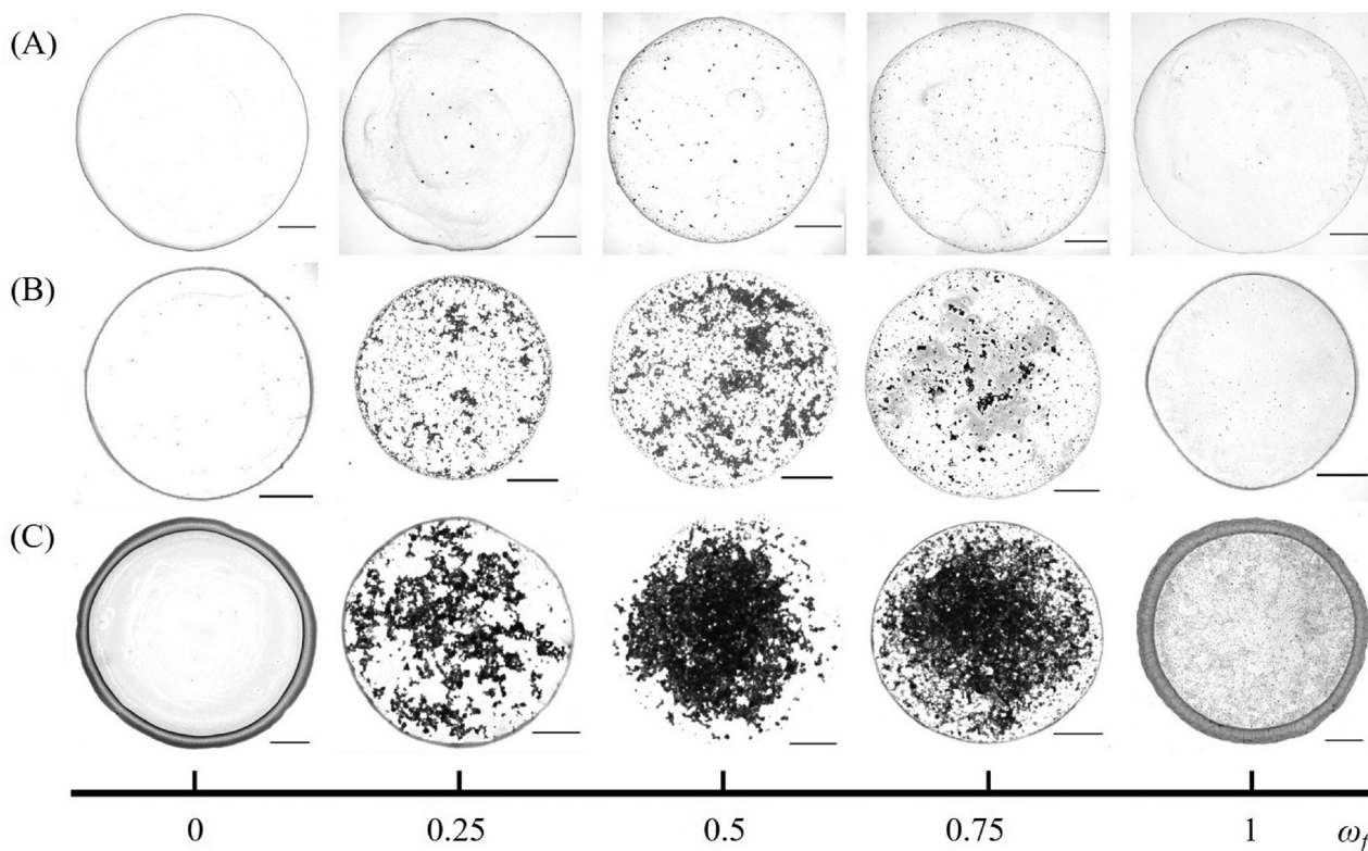
Fig. 1 Optical microscopy images of the dried deposit patterns formed by drying binary dispersions drops containing \text{PS}^+ - \text{PS}^- ( \approx 200 \text{ nm} diameter) at (A) C_T = 0.01\% , (B) C_T = 0.1\% , and (C) C_T = 1\% for various mixing fractions ( \omega_f ). The microscopy images shown have been recorded soon after complete evaporation of the liquid from the sessile drops, which had a typical lifetime of about 10 min. Scale bar = 500 \mu\text{m} .
