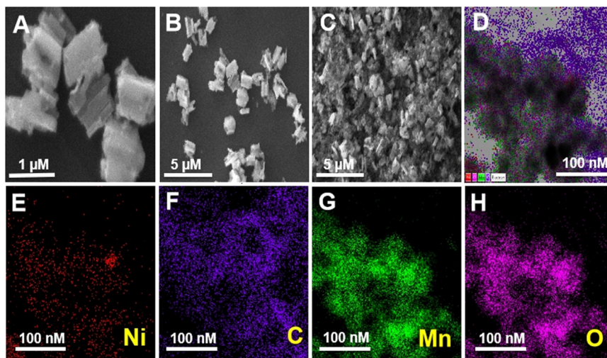
Fig. 2 SEM images of (A and B) \text{NiMn}_2\text{O}_4 at different magnification (C) \text{NiMn}_2\text{O}_4/\text{CNT} . (D–H) Elemental mapping analysis of the \text{NiMn}_2\text{O}_4/\text{CNT} nanocomposite showing elements Ni, C, Mn, and O.
