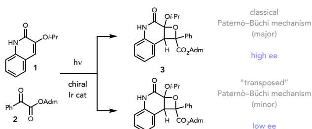
Figure 2. Prior work: detection of a minor transposed Paternò-Büchi pathway in asymmetric oxetane synthesis (Ref 9). Adm = adamantyl.
