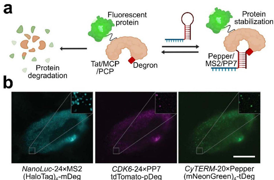
Fig. 8 (a) Schematic illustration of RNA-stabilized protein tags for live-cell RNA imaging. A protein destabilization degon domain is appended to the C-terminus of fluorescent protein-tagged Tat peptide or MS2/PP7 coat protein to induce protein degradation. While in the presence of a cognate pepper, MS2, or PP7 RNA motif, the degon can be shielded and thus stabilize the protein to generate localized fluorescence signals. (b) Orthogonal imaging of three different RNA species in live U2OS cells using MS2-mDeg (degon-appended MCP), PP7-pDeg (degon-appended PCP) and pepper-tDeg (degon-appended Tat peptide). Scale bar, 20 μm. Reproduced from ref. 131 with permission from the authors, copyright 2024.
