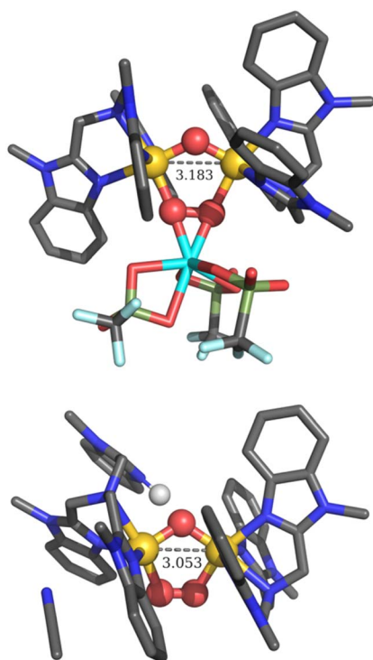
Fig. 3 Top: DFT optimized structure of 2+\text{Sc} . Bottom: DFT computed structure (r2scan-3c, COSMO) for 2+\text{H}^+ , which exhibits the short Fe...Fe distance as previously inferred from EXAFS analysis. 16
