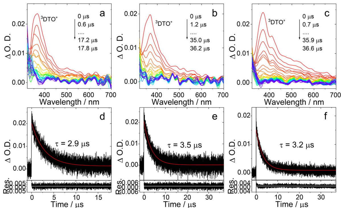
Fig. 7 Nanosecond transient absorption spectra of (a) PTZ-O-DTO, (b) PTZ-O 2 -DTP and (c) DPTZ-O-DTP. Decay traces of (d) PTZ-O-DTP, (e) PTZ-O 2 -DTP and (f) DPTZ-O-DTP at 370 nm after pulsed laser excitation at 355 nm. c = 2.0 \times 10^{-5} M in deaerated TOL, 25 °C.
