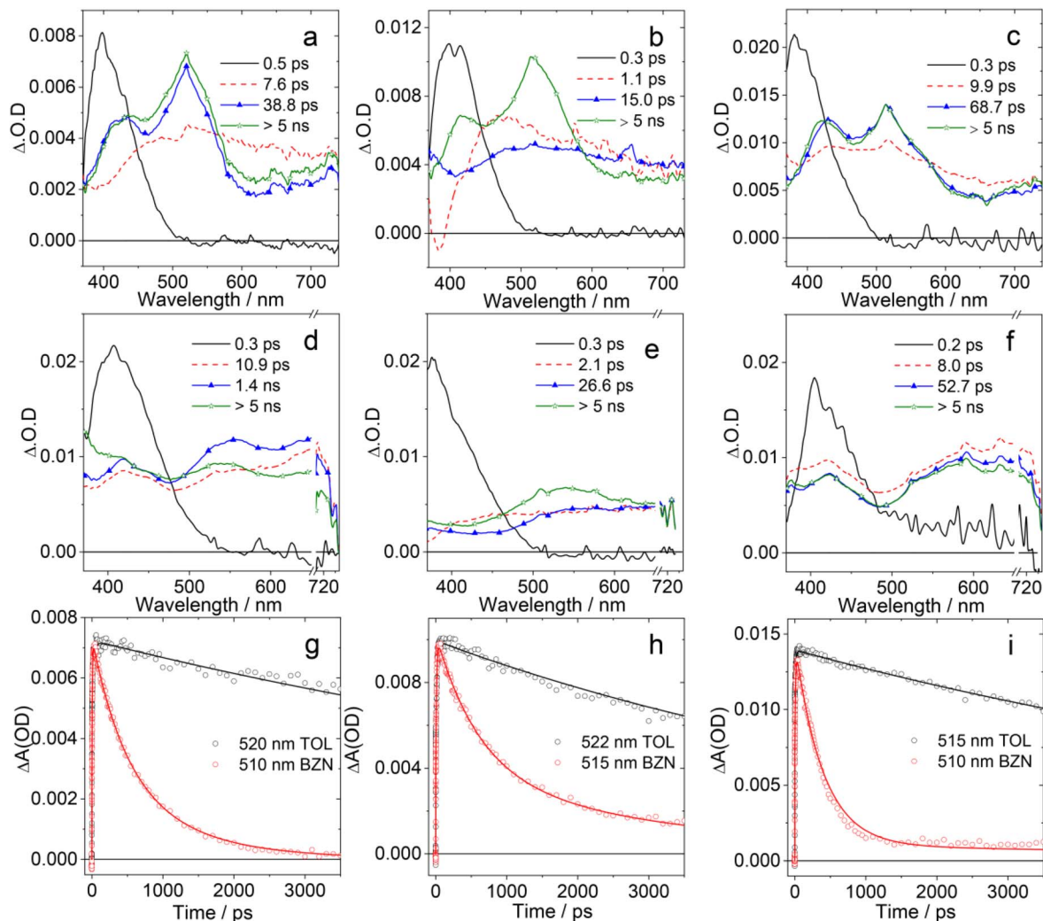
Fig. 5 EADS obtained from global analysis of the transient absorption data recorded for (a) PTZ-DTO, (b) PSeZ-DTO, (c) DPTZ-DTO, (d) PTZ-O-DTO, (e) PTZ-O 2 -DTO and (f) DPTZ-O-DTO in TOL upon excitation at 350 nm. Panels (g)–(i) report a comparison of the kinetic traces recorded at the maximum of the PTZ + signal for the three compounds presented in (a)–(c) in TOL and benzonitrile (BZN). The compounds were excited at 350 nm.
