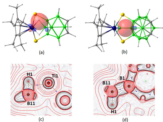
Fig. 6 Selected NBO of 3 showing (a) 3c–2e interaction of Ti1–H1–B11 and (b) 2c–2e interaction of B1–B11 (isocontour values: \pm 0.045 [e bohr ^{-3} ] ^{1/2} ). Contour-line diagram of the Laplacian of electron density along (c) Ti1–H1–B11 and (d) B1–B11–H1 planes in 3 .
