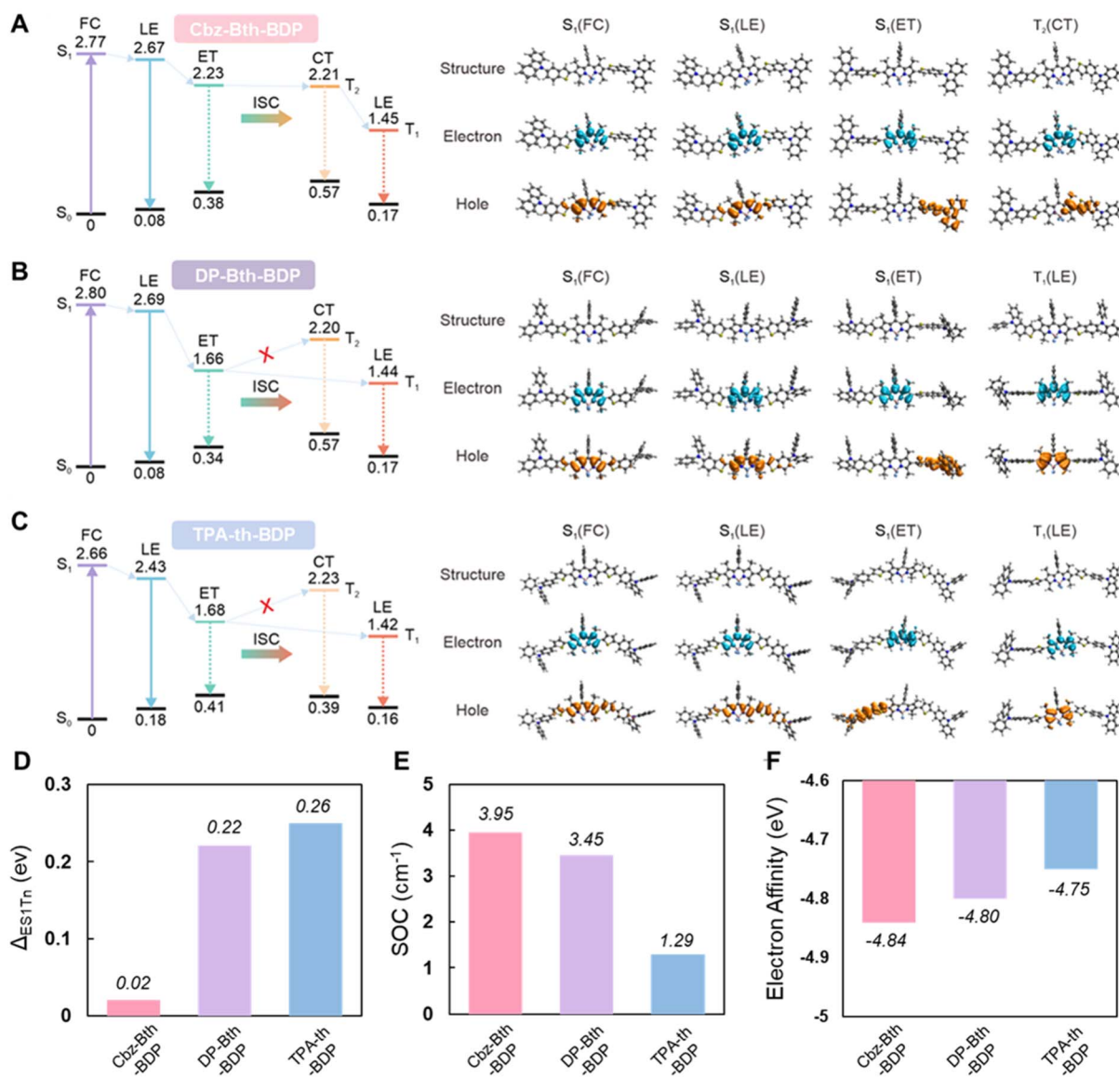
Fig. 2 Energy levels of key states, including the singlet Franck Condon (FC) state, locally excited (LE) state, electron transfer (ET) state, triplet LE, and charge-transfer ( T_1 and T_2 ) states. The molecular structures, and electron–hole distributions of S_1 (FC), S_1 (LE), S_1 (ET), T_2 (CT) and/or T_1 (LE) states for (A) Cbz-Bth-BDP, (B) DP-Bth-BDP, and (C) TPA-th-BDP. (D) The singlet–triplet energy gap ( \Delta E_{S1Tn} ), (E) spin–orbit coupling (SOC) values, and (F) theoretical electron affinities of thiophene-bridged BODIPY PSs.
