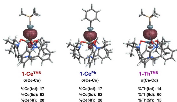
Fig. 5 Isosurfaces ( \pm 0.03 a.u.) of \sigma(Ce-C_\alpha) bonding NLMOs in 1-Ce TMS , 1-Ce Ph , and 1-Th TMS , along with total weight-% metal character and 6d vs. 5f contributions at the metal. (Color code: Ce yellow, Th sky blue, Si wheat, C gray, O red, N blue, and H white).
