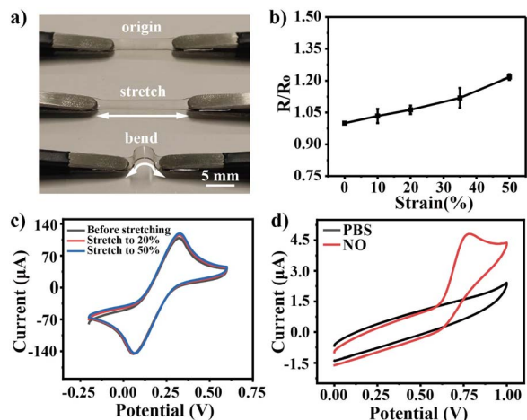
Fig. 2 Mechanical and electrochemical properties of PPL/PDMS. (a) Photographs of PPL/PDMS before and after deformation. (b) Resistance changes under 0–50% tensile strain ( n = 3 ). “ R ” represents the resistance of the stretched electrode, whereas “ R_0 ” denotes the resistance of the unstretched electrode. (c) CV curves of 10 mM K_3[Fe(CN)_6] on PPL/PDMS at different tension states from 0 to 50%. (d) CV curves of the electrode in PBS buffer salt solution with and without 180 \mu M NO.
