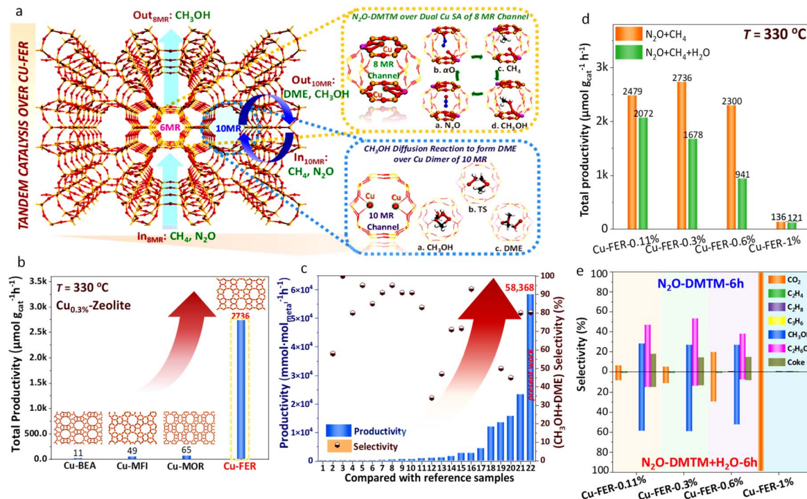
Fig. 1 Schematic diagram of \text{N}_2\text{O} -DMTM over Cu-FER and activity measurement results ( T = 330^\circ\text{C} and t = 6 h). (a) A dual Cu SA site can be formed at the opposite 6 MR of the \beta site of the 8 MR channel, efficiently favoring \alpha\text{O} formation, \text{CH}_4 activation and \text{CH}_3\text{OH} desorption. The \text{CH}_3\text{OH} would diffuse from the 8 MR channel into the 10 MR channel and readily react with \text{CH}_3^- and \text{OH}^- radicals, generated over the Cu dimer ( [\text{Cu}]^+ - [\text{Cu}]^+ ), to produce DME. (b) Total productivity ( \text{CH}_3\text{OH} + \text{DME} ) comparison over Cu-zeolite (BEA, MFI, MOR and FER) with Cu loading of 0.3 wt% (average value after 6 h reaction). (c) Productivity comparison with recent literature report of continuous DMTM (see Table S1†). (d) Total ( \text{CH}_3\text{OH} + \text{DME} ) productivity comparison over Cu-FER with diverse Cu loadings (0.11, 0.3, 0.6 and 1.0 wt%) in the absence and presence of \text{H}_2\text{O} (10 vol%). (e) Product selectivities corresponding to activity measurements in panel (d); reaction conditions: \text{N}_2\text{O}/\text{CH}_4/\text{He}/(\text{H}_2\text{O}) = 30:15:55(45):10 , with gas hourly specific velocity (GHSV) = 12\,000\text{ h}^{-1} , m_{\text{cat}} = 0.5\text{ g} ; other activity measurement results are profiled in Fig. S1a–e and 3a–f,† The total productivity, encompassing both \text{CH}_3\text{OH} and DME, was calculated by considering one mole of DME as equivalent to two moles of \text{CH}_3\text{OH} .
