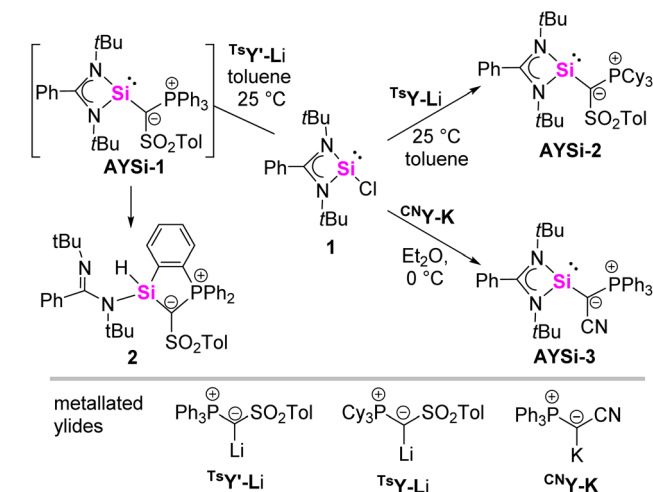
Scheme 1 Synthesis of the cyclic compound 2 and the amino(ylidyl)silylenes (AYSi) AYSi-2 and AYSi-3.
