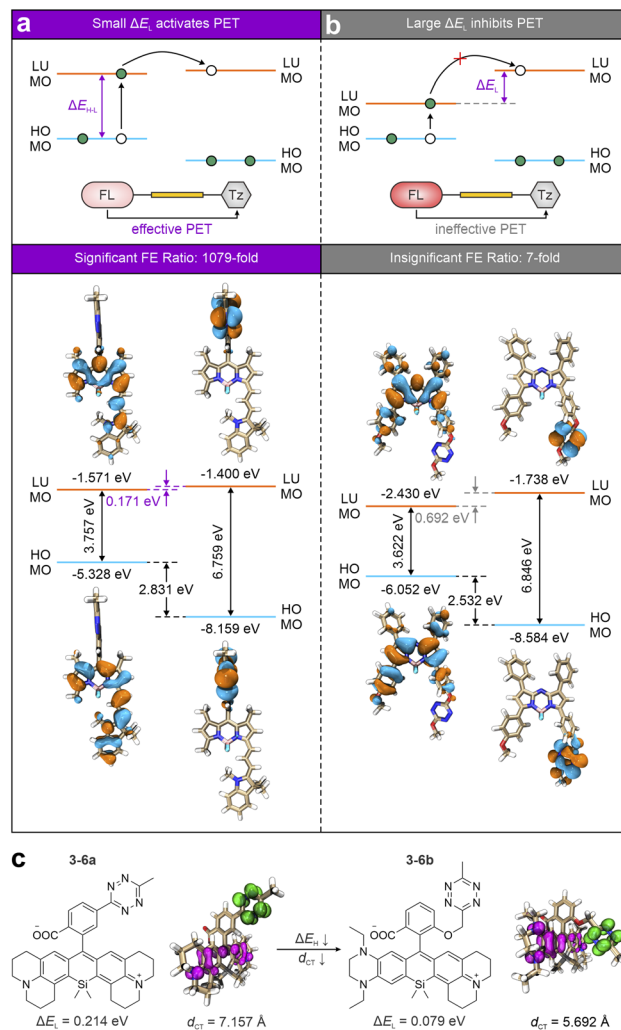
Fig. 9 Schematic illustrations of (a) effective and (b) ineffective PET activations based on the frontier molecular orbitals (top) with corresponding representatives of deep-red-to-NIR tetrazine-isolated labels. (c) Molecular structures and hole–electron distributions (top) with corresponding \Delta E_L and d_{CT} (bottom) of the ET states for 3-6a and 3-6b during the photoexcitation processes in DMSO. Hole – highlighted in pink; electron – highlighted in green. Reproduced with permission from ref. 54. Copyright 2024, The Royal Society of Chemistry.
