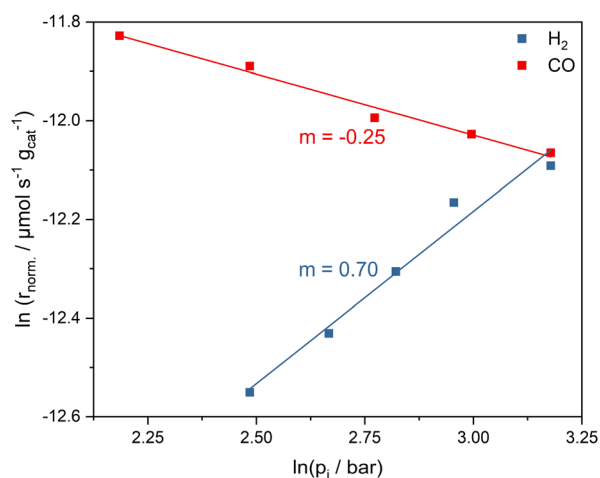
Fig. 6 Linearized plots of the logarithmic reaction rate r as a function of the CO and \text{H}_2 partial pressures and the derived reaction orders for CO and \text{H}_2 .
