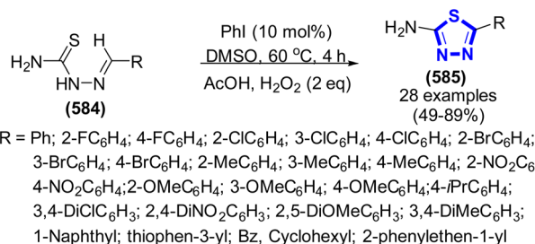
Scheme 157 Synthesis of 2-amino-1,3,4-thiadiazole catalyzed by PhI.
