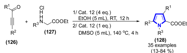
Scheme 35 Synthesis of polysubstituted pyrroles catalyzed by Cat. 12.
