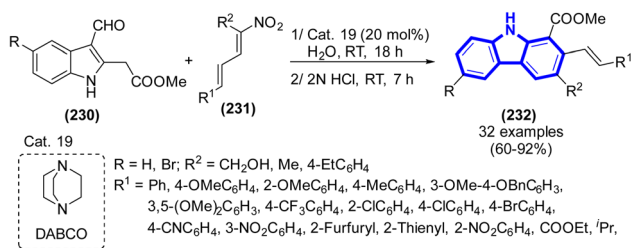
Scheme 63 Synthesis of substituted carbazoles catalyzed by Cat. 19.
