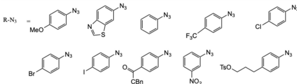
Scheme 62 Microwave-assisted synthesis of 1,2,3-triazoles (73a–k). 109
