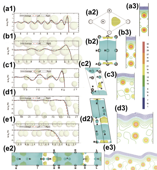
Fig. 30 Friedel oscillations as a function of the depth z are shown for (a1) Mg(0001), (b1) Mg(1010), (c1) Mg(1011), (d1) Mg(1013) and (e1) Mg(1018). Subsequent top-down views of charge transfer are presented for (a2) Mg(0001), (b2) Mg(1010), (c2) Mg(1011), (d2) Mg(1013) and (e2) Mg(1018). Cross-sectional views of charge densities are displayed for (a3) Mg(0001), (b3) Mg(1010), (c3) Mg(1011), (d3) Mg(1013) and (e3) Mg(1018). The topmost surface layer is indicated with an underline. In the charge transfer sections specifically in graphs (a2), (b2), (c2), (d2), and (e2) light blue and yellow squares represent charge depletion and accumulation in the surface region. The color bar illustrates the logarithmic range of charge densities from low (blue 1) to high (red 30), and the charge density value for a specific line can be obtained by the formula \rho = 0.001 \times 2^{n/2} . Reprinted with permission from the work of Tang et al. 154
