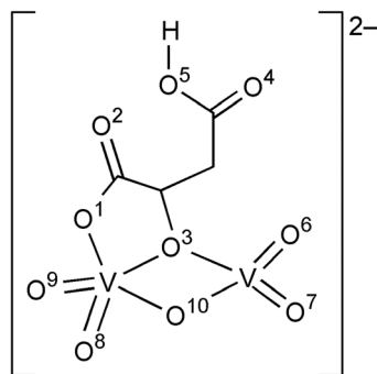
Fig. 8 Structure of [V_2^V O_5(mal)]^{2-} complex.
