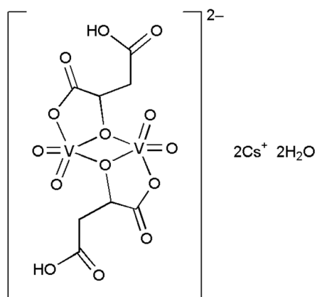
Fig. 1 Structure of Cs 2 [V 2 O 4 (mal) 2 ]·2H 2 O.
