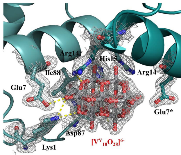
Fig. 9 Vanadium binding sites in structure B: non-covalent interaction of the [V_{10}^V O_{28}]^{6-} to the protein surface. 2Fo-Fc electron density maps are reported at 1.0\sigma level in grey. Asterisk refers to atoms from symmetry-related molecules (deep teal). Anomalous difference electron density map is reported in Fig. S4B.†
