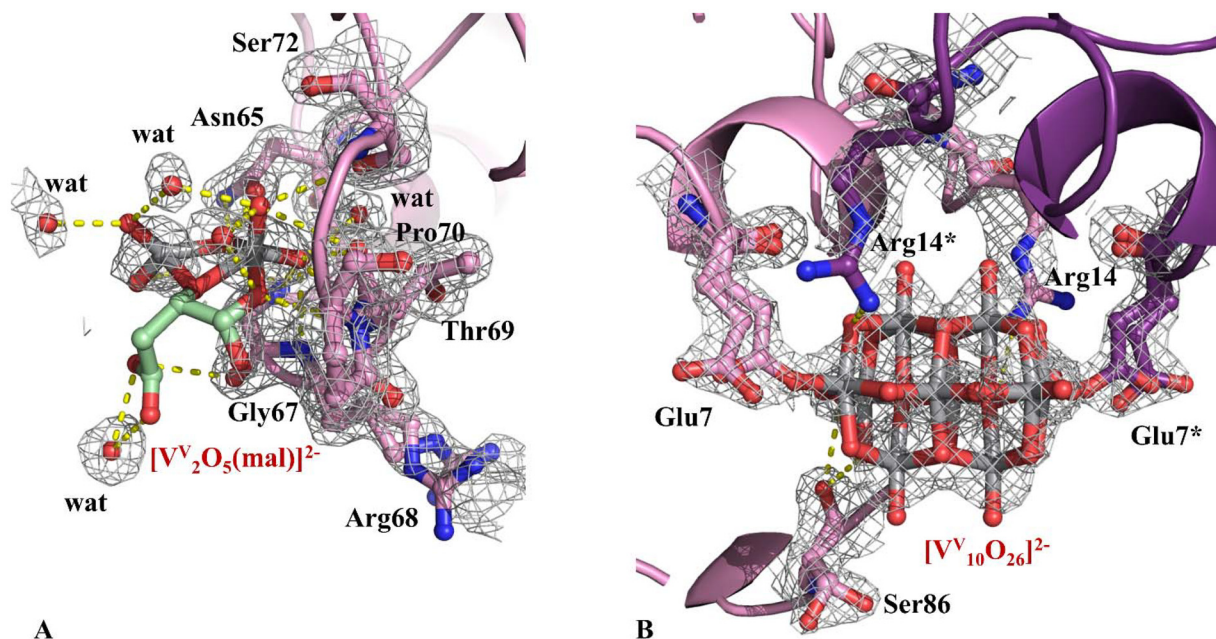
Fig. 7 Vanadium binding sites in the structure A: (A) non-covalent interaction of the dinuclear oxidovanadium(V) complex [V_2^V O_5(mal)]^{2-} to the protein surface; (B) covalent binding of the [V_{10}^V O_{26}]^{2-} to the side chain of Glu7 and Glu7*. 2Fo-Fc electron density maps are reported at 1.0\sigma level in grey. Anomalous difference electron density map is reported in Fig. S4A.† Asterisk refers to atoms from symmetry-related molecules (coloured in purple). Glu7 and Arg86 side chains adopt two alternative conformations.
