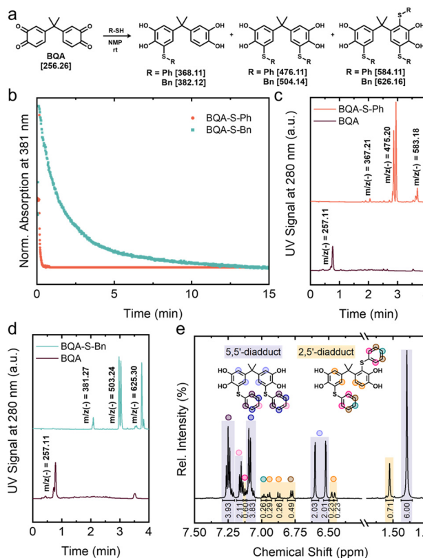
Fig. 2 Michael-type model reactions of BQA with either Ph-SH or Bn-SH. The corresponding exact masses (Da) are shown in brackets (a). UV/vis spectroscopy following the consumption of BQA by monothiols (b). UHPLC UV traces of the reaction mixture of BQA with Ph-SH (c) or with Bn-SH (d) after 12 h reaction (solvent A: water, 0.1% formic acid, solvent B: acetonitrile, 0.1% formic acid, gradient 30–90% B; with BQA reference). 1 H NMR spectroscopy of BQA/2Ph-SH reaction assigned to 5,5'-diadducts (violet) and 2,5'-diadducts (yellow) (e).
