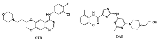
Scheme 1 Chemical structures of gefitinib (GTB) and dasatinib (DAS).
