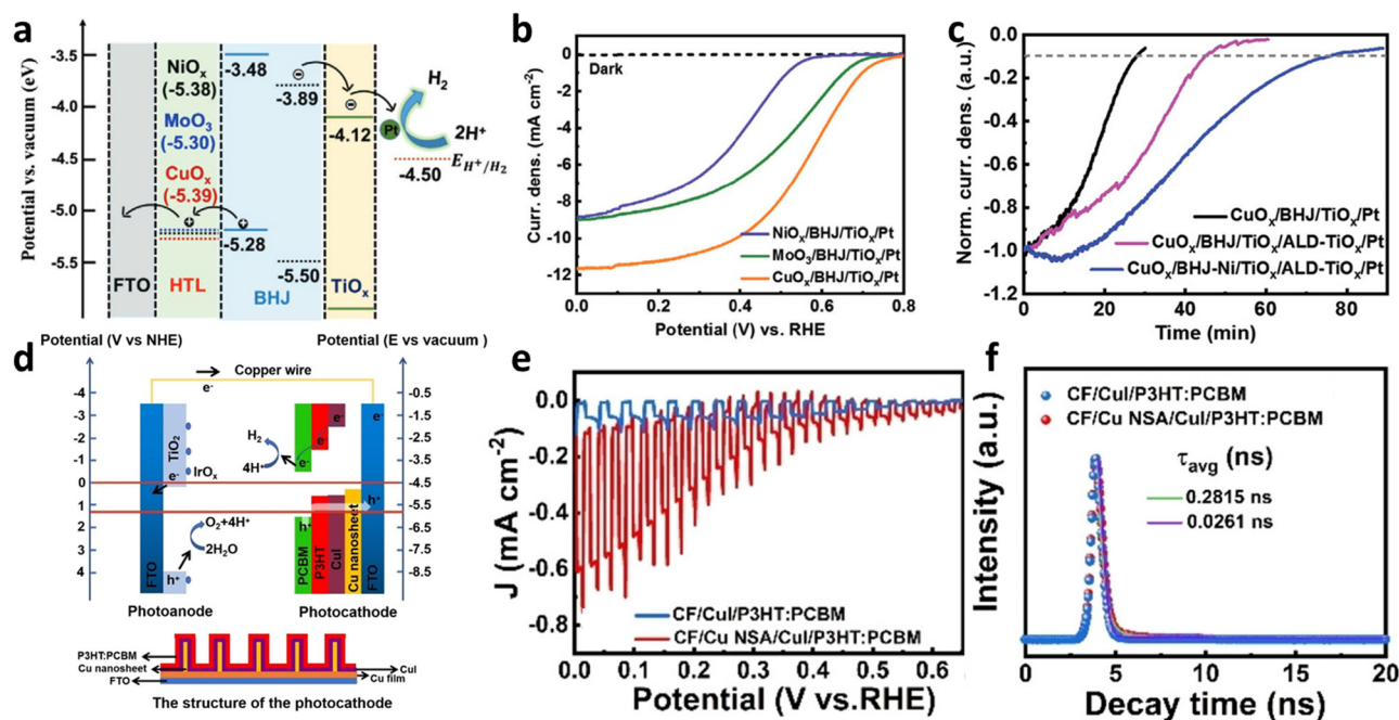
Fig. 6 (a) Energy level diagram of the photocathode based on the non-fullerene BHI (PBDB-T:ITIC). (b) LSV curves of the photocathodes with the various HTLs and (c) stability test of the different photocathode at 0 V RHE in 0.1 M H 2 SO 4 buffer adjusted to pH 1. Adapted with permission. Adapted with permission. 50 Copyright 2020, Wiley-VCH GmbH. (d) Energy level alignment of Cu nanosheet (Cu NSA)-fabricated photocathode and photoanode (above) with the structure of the photocathode (below). (e) Chopped J-V curves and (f) time-resolved transient PL spectra of the photocathodes with and without Cu NSA. Adapted with permission. 54 Copyright 2021, Wiley-VCH GmbH.
