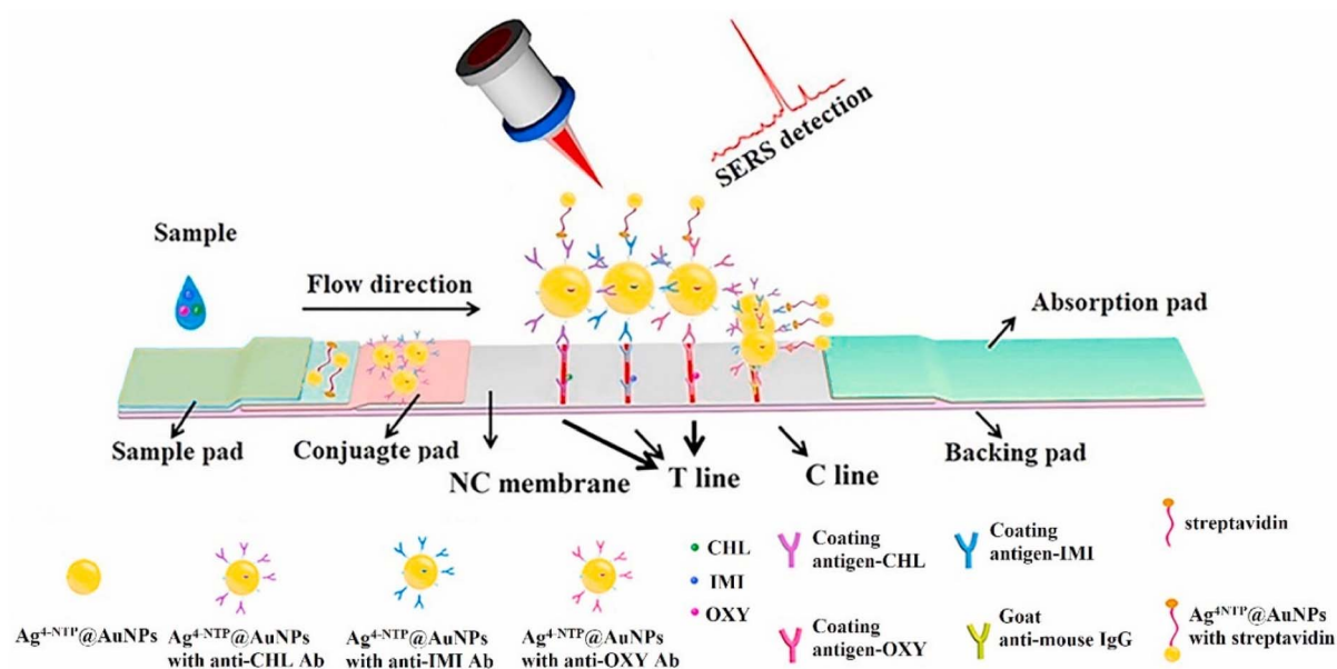
Fig. 12 Scheme of the LFA-SERS strategy using enhanced \text{Ag}^4\text{-NTP@Au} for the multiplex strip. This figure has been adapted/reproduced from ref. 189 with permission from Elsevier, copyright 2025.
