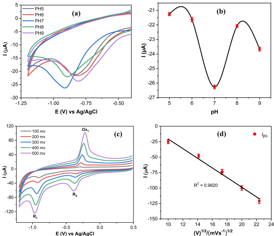
Fig. 9 (a) CV curves obtained at AgNPs@GO/IL@SPCE in 0.1 mol L -1 PBS containing 20 \mu\text{mol L}^{-1} MP at different pH; scan rate 100 mV s -1 . (b) The correlation between the pH and the reduction peak current of MP. (c) CV curves of 20 \mu\text{mol L}^{-1} PM in 0.1 mol L -1 PBS (pH 7) at different scan rates. (d) A graph depicting the peak currents of MP reduction ( R_1 ) plotted against the square root of the scan rate. Note: geometric area of the working electrode: 7 mm 2 .
