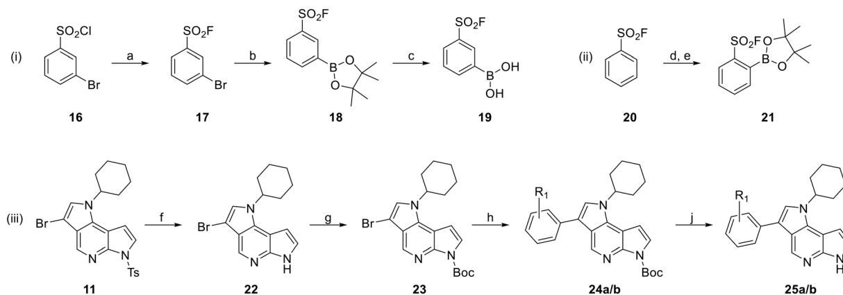
Scheme 2 Synthesis of compounds 25a/b . Reagents and conditions: (i) synthesis of (3-(fluorosulfonyl)phenyl)boronic acid ( 19 ): (a) \text{KHF}_2 , \text{MeCN}/\text{H}_2\text{O} (2 : 1, V/V), rt, 24 h, quant.; (b) \text{B}_2\text{pin}_2 , KOAc, \text{Pd}(\text{dppf})\text{Cl}_2 , dioxane, 80 °C, 16 h, 79%; (c) \text{NH}_4\text{OAc} , \text{NaIO}_4 , acetone/ \text{H}_2\text{O} (1 : 1, V/V), rt, 30 h, 75%; (ii) synthesis of para -analog 21 : (d) LDA, \text{B}(\text{O}^i\text{Pr})_3 , THF, -78 °C, 2 h; then (e) pinacol, toluene, rt, 22 h, 39%; (iii) synthesis of final compounds 25a/b : (f) KOH, MeOH, rf, 3 h, 62%; (g) \text{Boc}_2\text{O} , DMAP, TEA, DCM, rt, 2 h, 96%; (h) for \text{R}_1 = m\text{-SO}_2\text{F} (a): 19 , \text{K}_3\text{PO}_4 , \text{Pd}(\text{OAc})_2 , XPhos, dioxane/ \text{H}_2\text{O} (2 : 1, V/V), 40 °C, 4 h, 54%; for \text{R}_1 = o\text{-SO}_2\text{F} (b): 21 , KF, \text{Pd}(\text{OAc})_2 , XPhos, THF, 40 °C then rt, 20 h, 32%; (j) HCl in dioxane (4 M), rt, 18–20 h, 32–95%.
