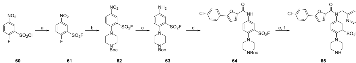
Scheme 6 Synthesis of compound 65 . Reagents and conditions: (a) \text{KHF}_2 , MeCN/ \text{H}_2\text{O} (2 : 1, V/V), rt, 18 h, quant.; (b) 1-Boc-piperazine, DIPEA, DMF, 80 °C, 3 h, 54%; (c) Pd/C, \text{H}_2 , MeOH, rt, 1 h, quant.; (d) 5-(4-chlorophenyl)furan-2-carboxylic acid, HATU, DIPEA, DMF, 80 °C, 17 h, 37%; (e) 2-(bromomethyl)pyridine HBr, NaH, DMF, rt, 20 h; then (f) TFA, DCM, rt, 2 h, 42% over two steps.
