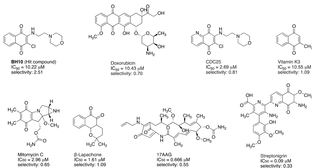
Fig. 2 Chemical structure and biactivity of BH10 and seven other well-known anticancer compounds. IC_{50} values ( \mu M ) indicate the cytotoxicity towards HEC1A endometrial cancer cells, while selectivity is calculated as the IC_{50} value for non-cancerous MAD11 cells divided by the IC_{50} value for HEC1A cells. 7
